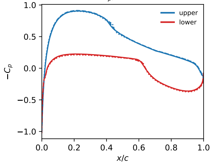
C_p, \alpha = 0^\circ
