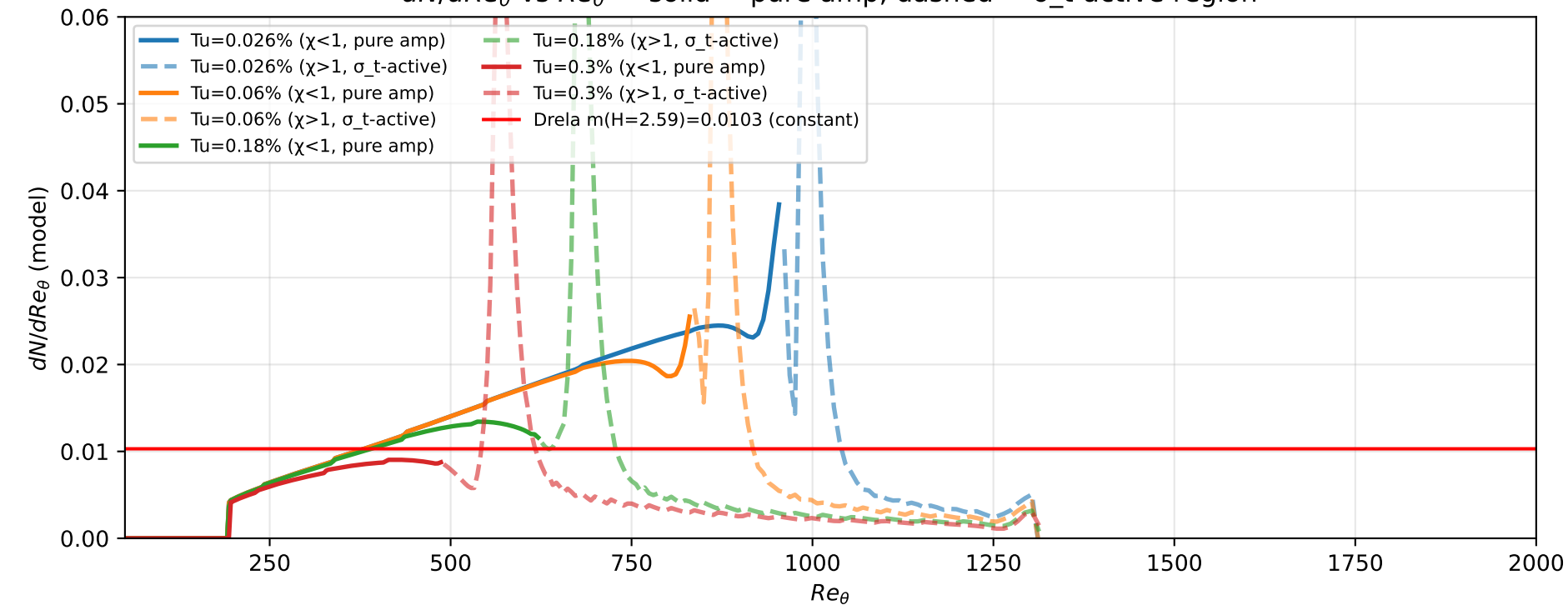
dN/dRe_\theta vs Re_\theta — solid = pure amp, dashed = \sigma_t -active region
