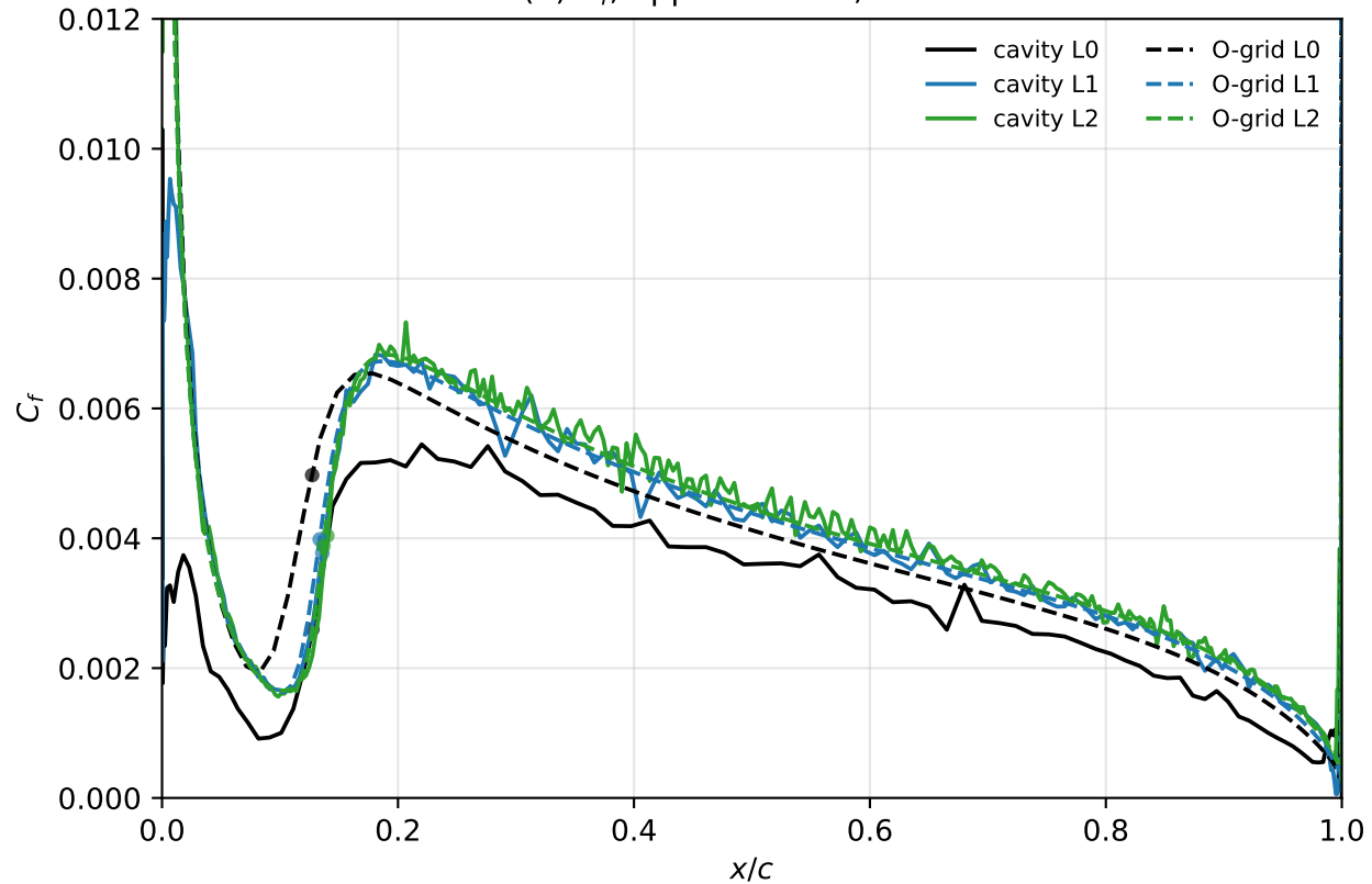
(b) C_f , upper surface, \alpha = 4^\circ
