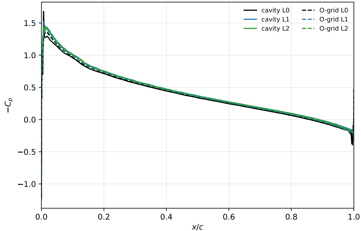
(a) C_p , upper surface, \alpha = 4^\circ
