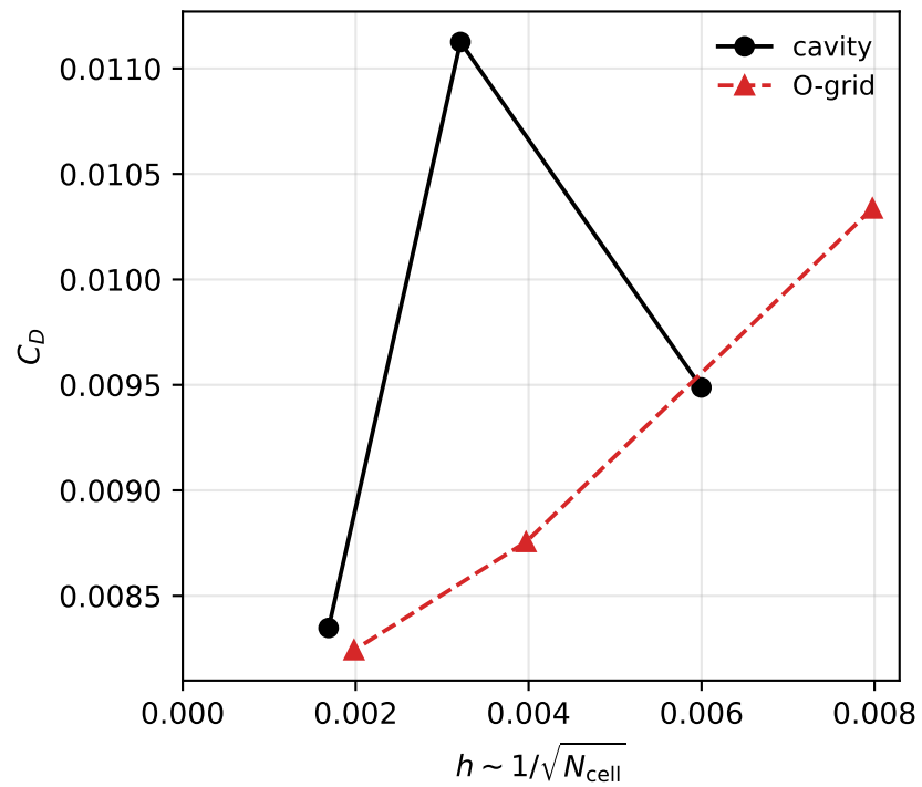
(b) drag coefficient
