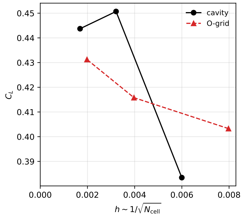
(a) lift coefficient
