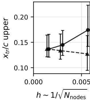
(g) suction-side transition
