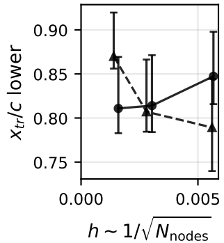
(g) suction-side transition
