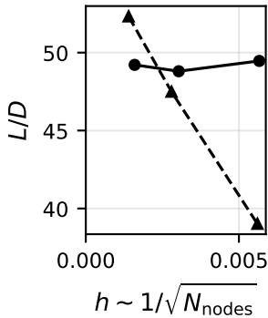
(f) lift-to-drag ratio
