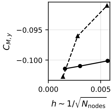
(e) pitching moment
