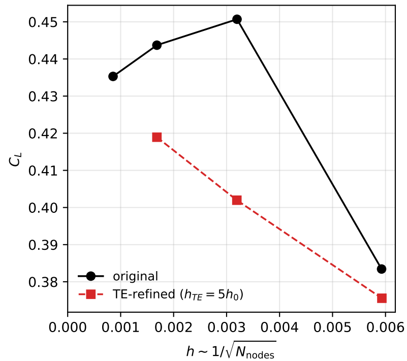
(a) lift
