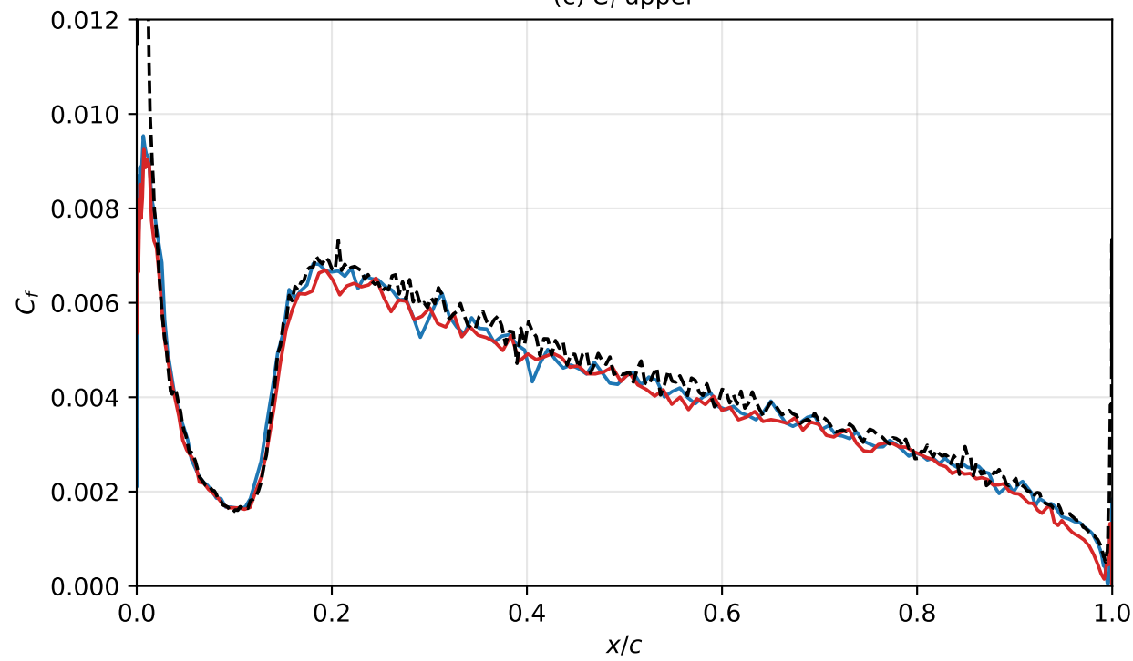
(c) C_f upper
