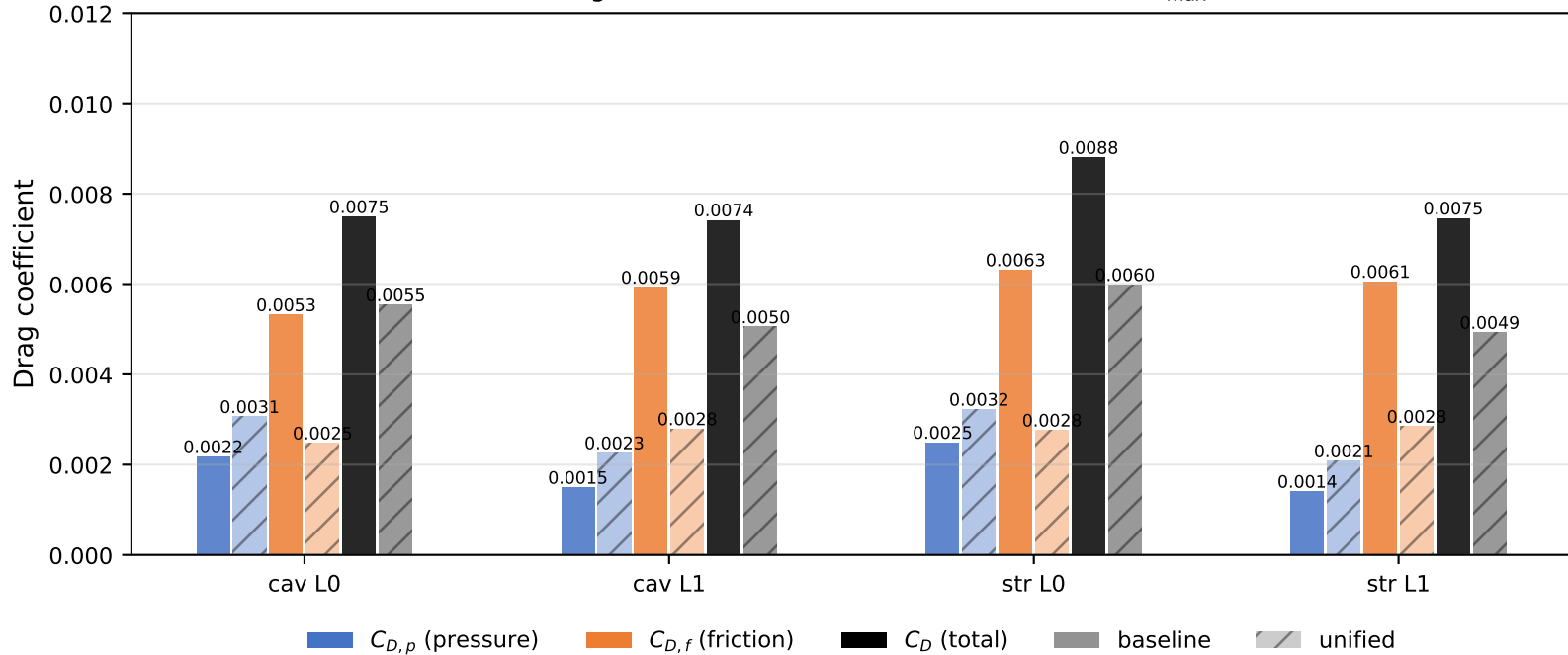
NACA 0012 \alpha = 0^\circ : drag breakdown — baseline (solid) vs unified a_{\max} = 0.2 (hatched)
