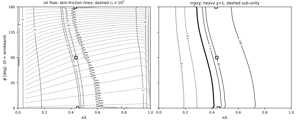
Figure 27: \alpha = 2.5^\circ , Re_L = 7.2 \times 10^6 .
