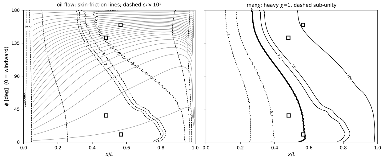
Figure 29: \alpha = 5^\circ , Re_L = 6.49 \times 10^6 .
