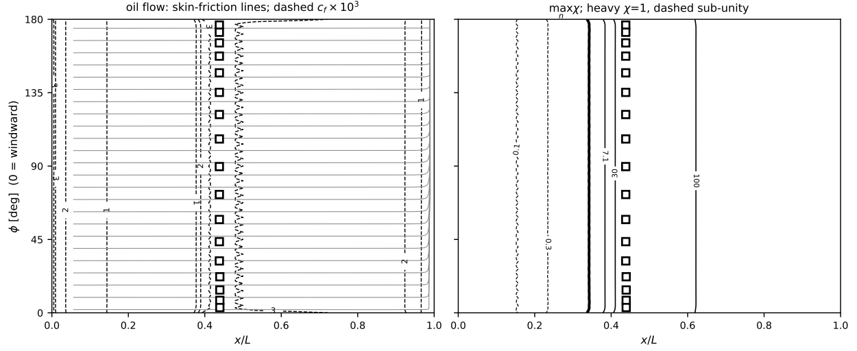
Figure 26: Surface at the measured-seed condition, unrolled into (x/L, \phi) , \phi = 0 windward; line art throughout. Left: the oil-flow analogue – grey skin-friction lines integrated from the wall shear vector itself, not the inviscid streamlines of Stock Figs. 14–17 – with |c_f| \times 10^3 as black dashed contours; streak convergence is the separation signature. Right: \max_n \chi on a wall-normal segment shot from each surface point, sub-unity decades dashed, \chi = 1 heavy, \chi = c_{v1} and above solid. White-filled squares: measured DFVLR transition. \alpha = 0^\circ , Re_L = 7.2 \times 10^6 .
