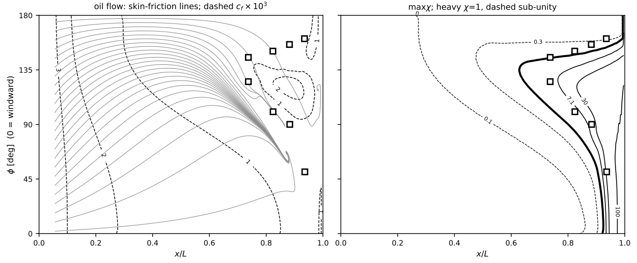
Figure 28: \alpha = 5^\circ , Re_L = 1.52 \times 10^6 .
