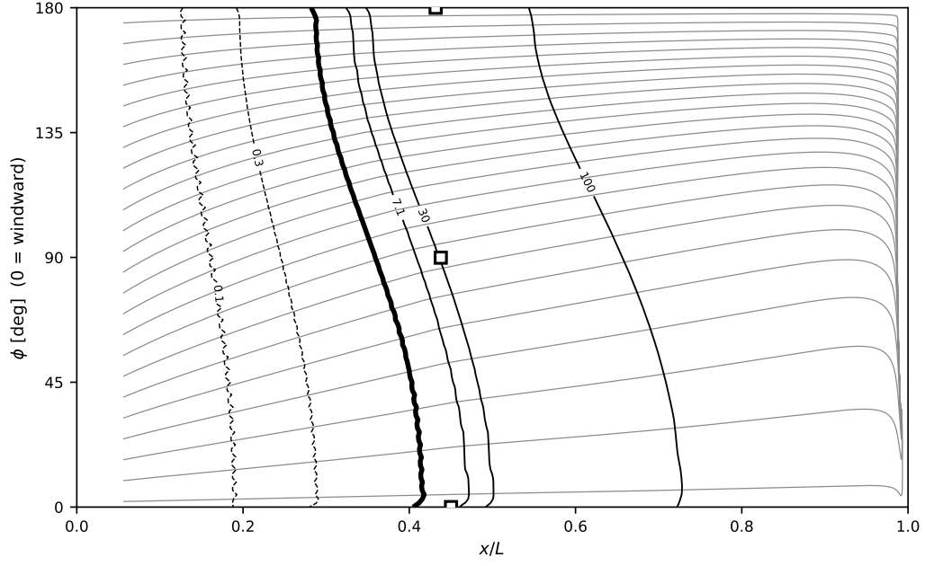
Figure 37: The two views superposed, inclined conditions. Grey skin-friction lines under the \max_n \chi contour family (sub-unity dashed, \chi = 1 heavy, \chi = c_{v1} and above solid, labeled); white-filled squares measured DFVLR transition. Zero incidence is omitted: both views are functions of x/L alone there. \alpha = 2.5^\circ , Re_L = 7.2 \times 10^6 .
