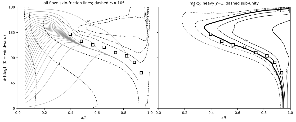
Figure 30: \alpha = 10^\circ , Re_L = 1.52 \times 10^6 .
