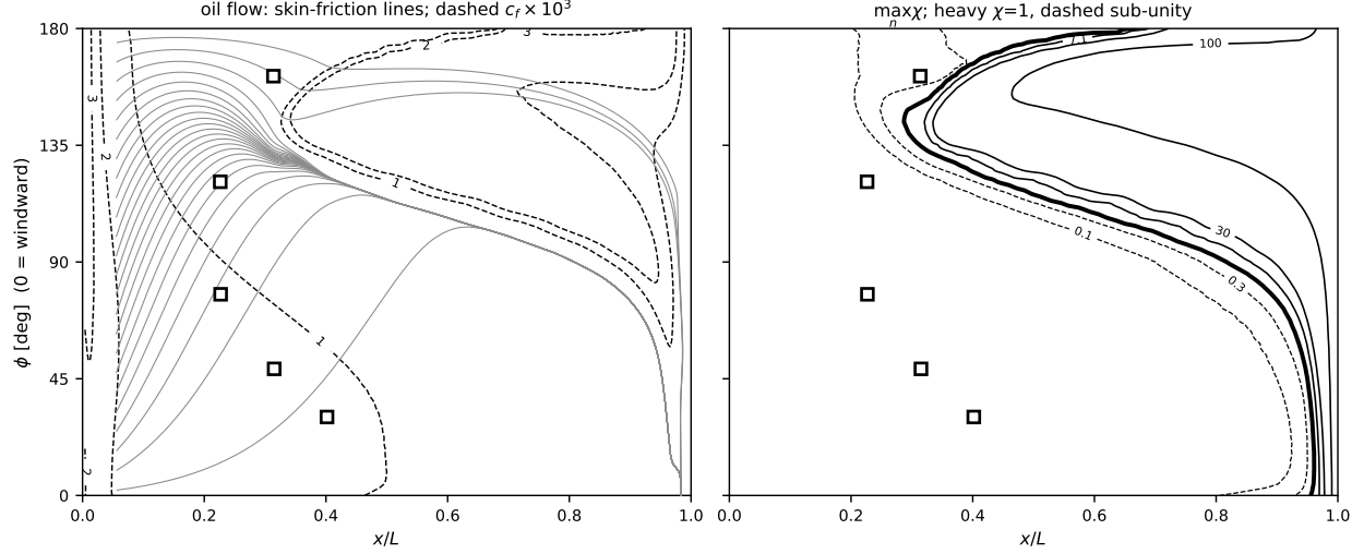
Figure 32: \alpha = 10^\circ , Re_L = 6.56 \times 10^6 , ONERA F1.
