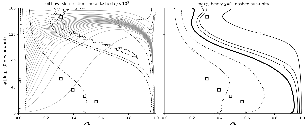
Figure 31: \alpha = 10^\circ , Re_L = 6.56 \times 10^6 , Göttingen.
