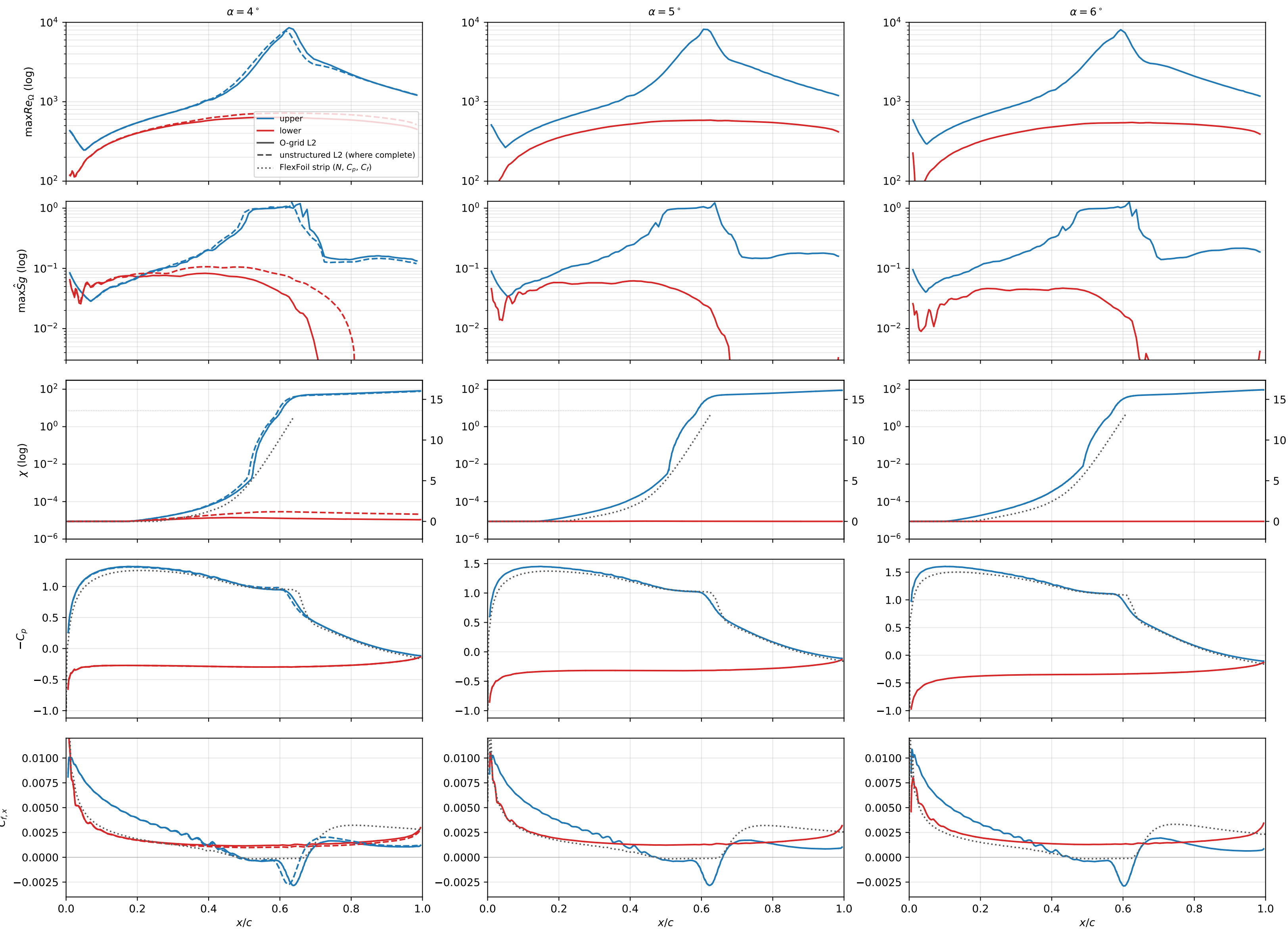
Daedalus wing section \eta = 0.60 ( Re_c = 5e + 05 )
