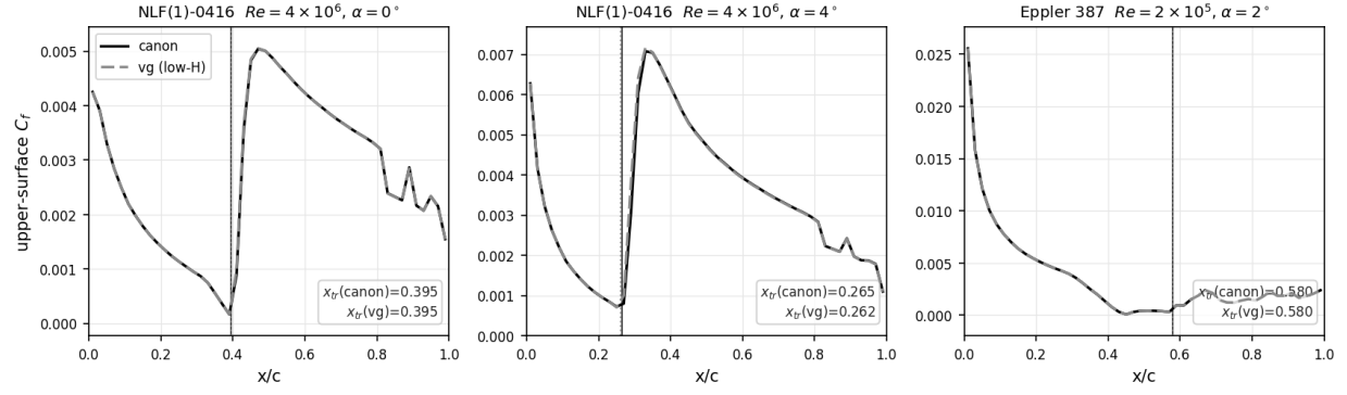
Figure 30: Upper-surface C_f(x/c) , canon (black) vs vg low- H (gray dashed), kernel-only delta (same mesh/config/seed, vg warm-restarted from canon). Vertical ticks: transition front (near-wall \chi = 1 for NLF, C_f -rise for Eppler). Curves and fronts overlap: NLF(1)-0416 Re = 4 \times 10^6 \alpha = 0^\circ x_{tr} = 0.395 (both), \alpha = 4^\circ 0.265 \rightarrow 0.262 ; Eppler 387 Re = 2 \times 10^5 \alpha = 2^\circ 0.580 (both). The low- H branch does not trip the favorable rooftop.
