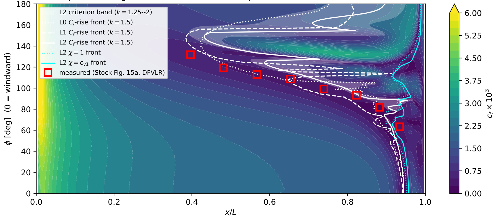
6:1 spheroid, Re_L = 1.5 \times 10^6 , \alpha = 10^\circ : computed fronts vs measured transition
