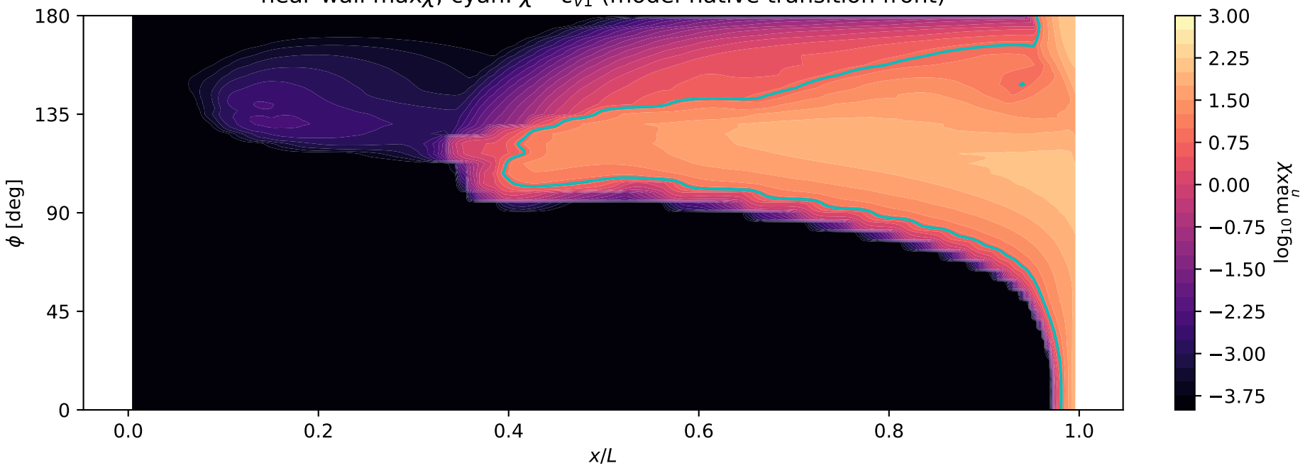
near-wall \max \chi ; cyan: \chi = c_{v1} (model-native transition front)
