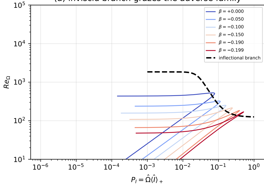
(a) inviscid branch grazes the adverse family
