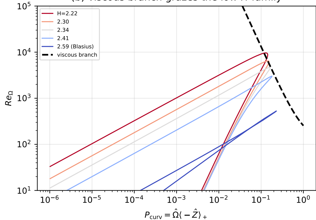
(b) viscous branch grazes the low- H family
