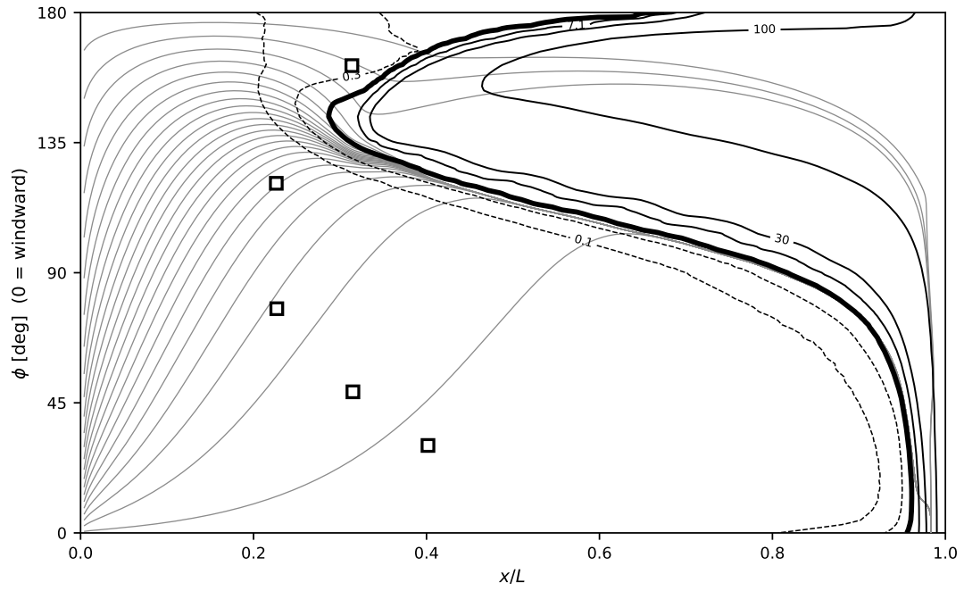
Figure 33: \alpha = 10^\circ , Re_L = 6.56 \times 10^6 , ONERA F1.
