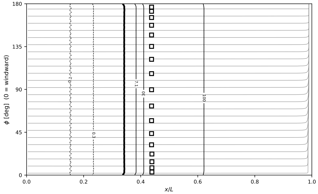
Figure 29: \alpha = 0^\circ , Re_L = 7.2 \times 10^6 .
