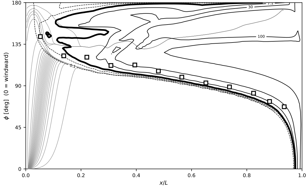
Figure 28: \alpha = 29.7^\circ , Re_L = 1.53 \times 10^6 ; the friction lines converge onto the open free-vortex-layer separation over most of the leeward half, and the twelve measured stations lie on that line rather than on a transition front.
