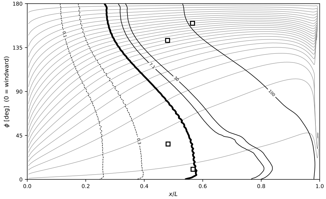
Figure 31: \alpha = 5^\circ , Re_L = 6.49 \times 10^6 .
