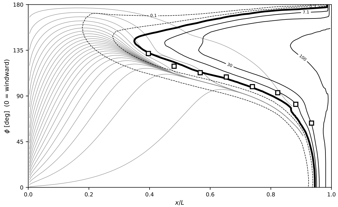
Figure 27: \alpha = 10^\circ , Re_L = 1.52 \times 10^6 .
