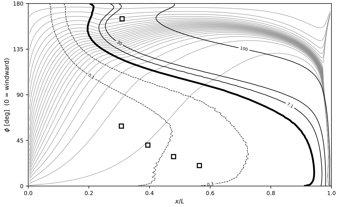
Figure 32: \alpha = 10^\circ , Re_L = 6.56 \times 10^6 , Göttingen.
