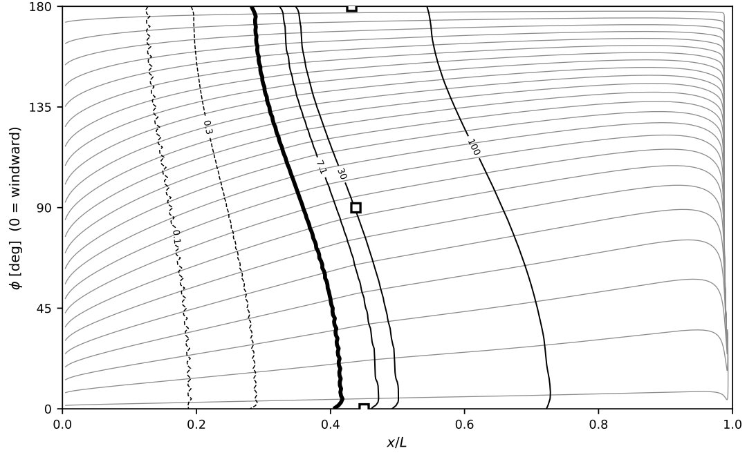
Figure 30: \alpha = 2.5^\circ , Re_L = 7.2 \times 10^6 .
