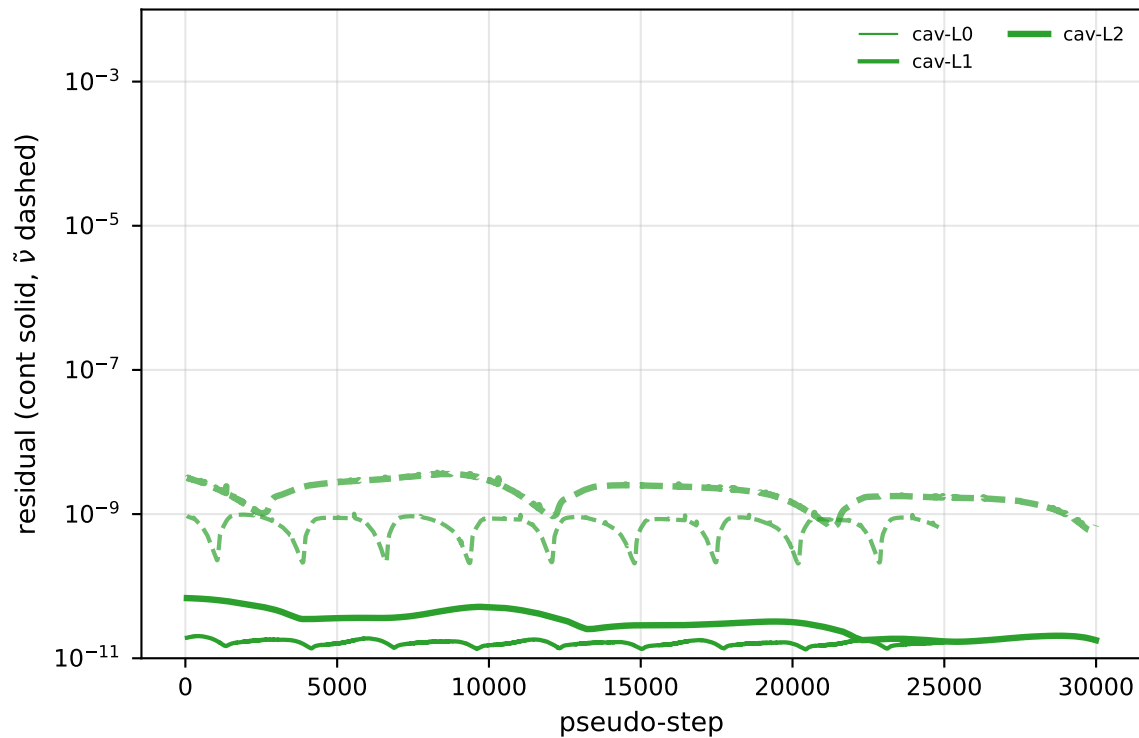
\alpha=8.5^\circ : residuals
