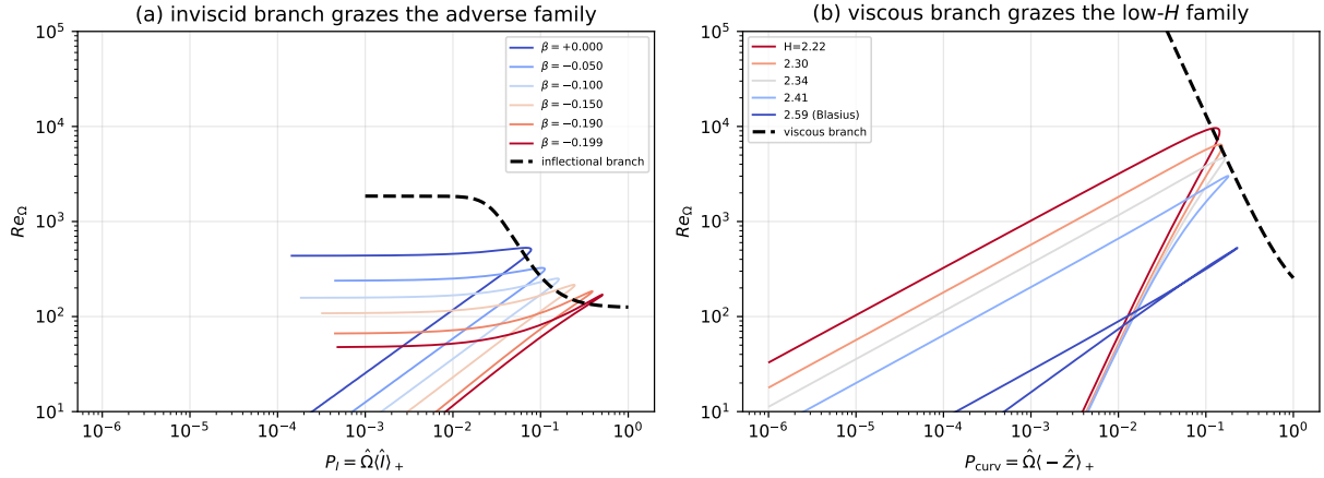
Fig. H6 Each onset branch grazes its own family in its own coordinate, each profile evaluated at its Drela–Giles critical Reynolds number Re_{\theta 0}(H) . (a) the inflectional branch A + B/P_I^2 against the adverse family; the strongly favorable members collapse to P_I \rightarrow 0 and leave the panel, which is the onset-resolution limit of a single-coordinate gate. (b) the curvature branch A + B_c/P_c^2 against exactly those low- H members, in the coordinate P_c of Eq. (E5).
