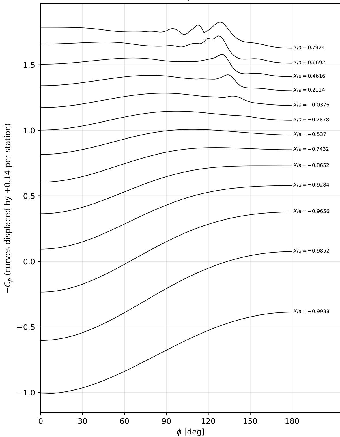
\alpha = 10^\circ , Re_L = 1.5 \times 10^6 (L2): C_p at the DFVLR pressure stations
