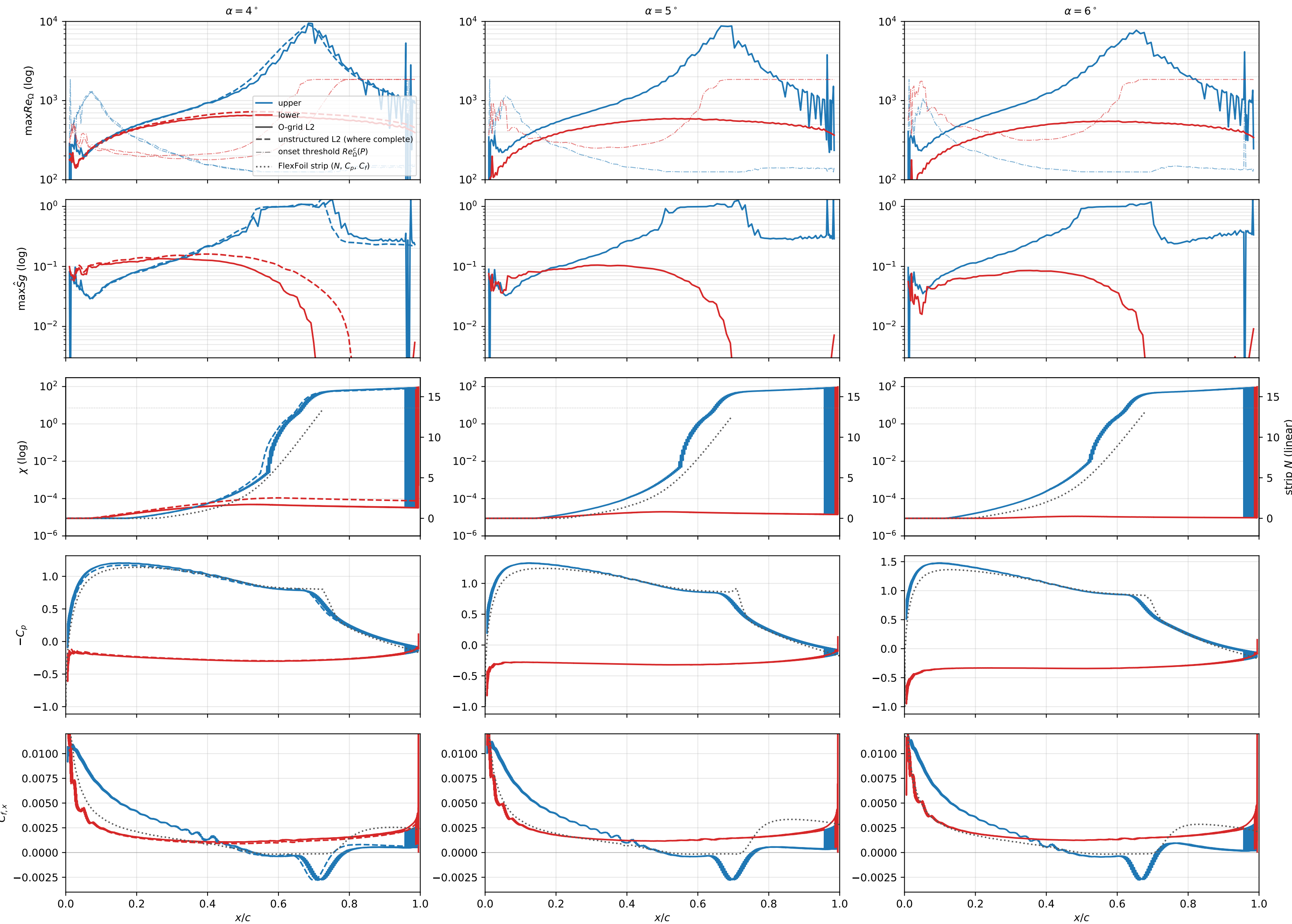
Daedalus wing section \eta = 0.92 ( Re_c = 4e + 05 )
