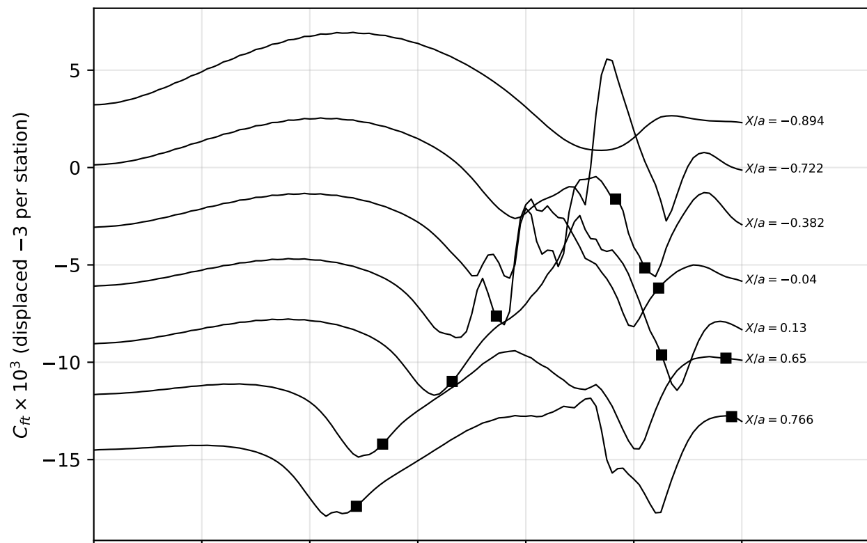
\alpha = 29.7^\circ , Re_L = 1.5 \times 10^6 (L2): wall shear at the DFVLR hot-film stations
