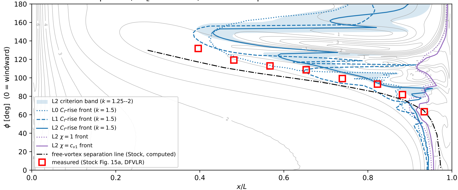
6:1 spheroid, Re_L = 1.5 \times 10^6 , \alpha = 10^\circ : computed fronts vs measured transition
