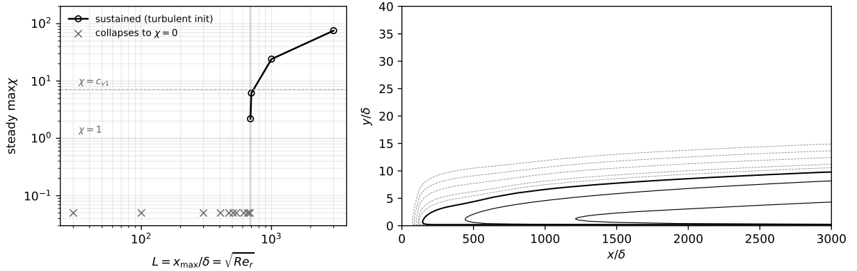
Figure 5: Attachment-anchored turbulent branch. Standard SA, frozen Hiemenz, \chi_\infty = 0 ; laminar for L \lesssim 685 , critical band Re_r = 4.66\text{--}4.74 \times 10^5 , \max \chi \approx 0.025 L . Right: L = 3000 ( Re_r = 9 \times 10^6 ), \max \chi = 76 ; \log_{10} \chi contours dashed below \chi = 1 , solid at 1, c_{v1} , 30. \max \chi \approx 24 at Re_r = 10^6 , 76 at 9 \times 10^6 .
