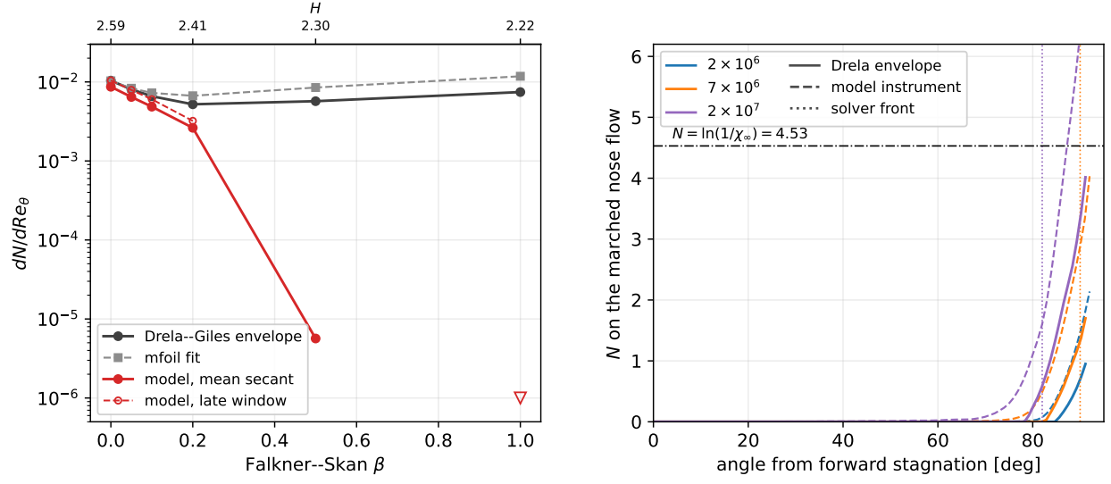
Figure 22: Favorable-gradient amplification audit; cylinder nose at Re_D = 2 \times 10^6 , 7 \times 10^6 , 2 \times 10^7 (middle seed), transition budget N = \ln(1/\chi_\infty) = 4.53 .
