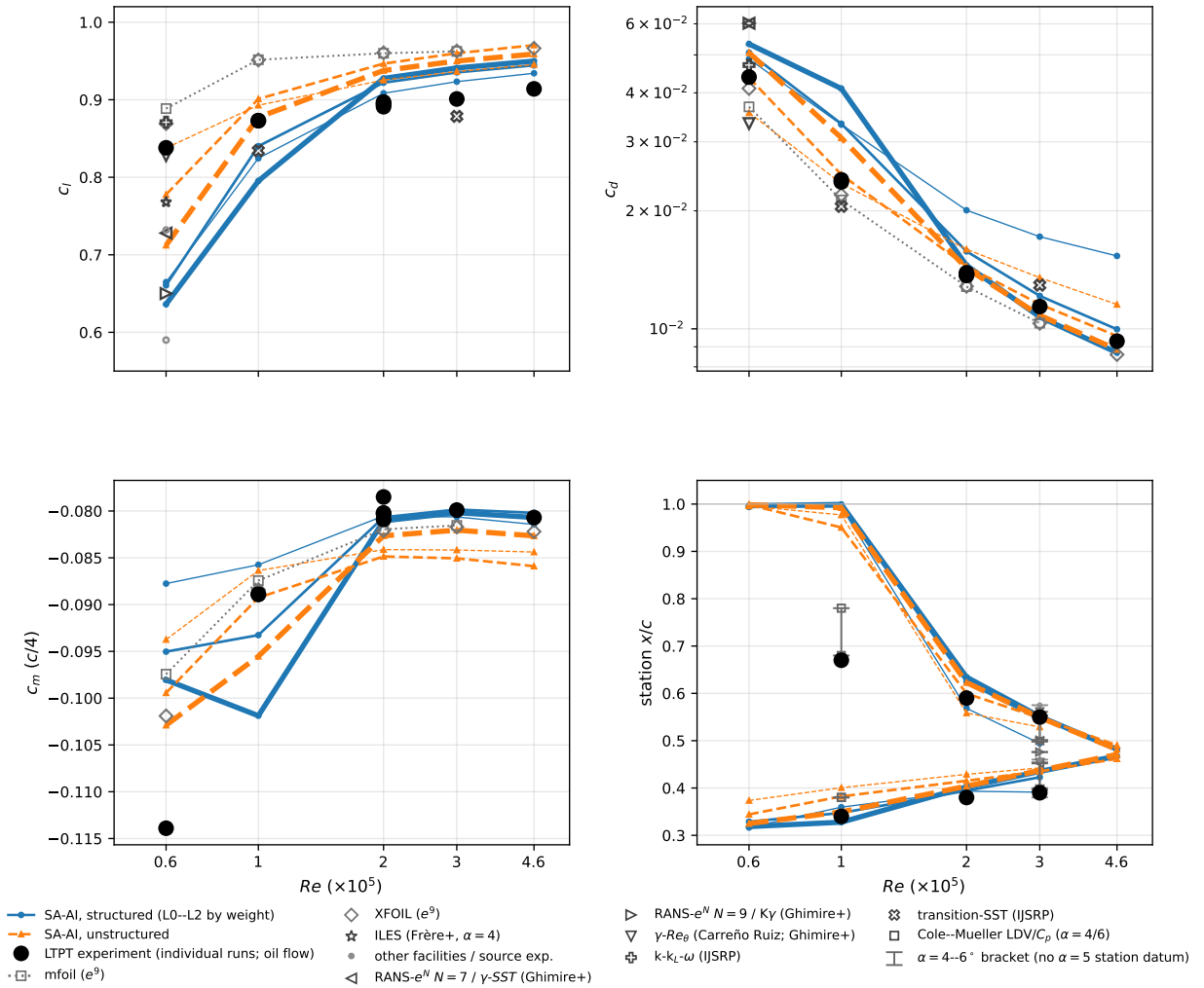
Figure 17: Reynolds-sweep forces and stations, \alpha = 5^\circ , Re = 6 \times 10^4\text{--}4.6 \times 10^5 . LTPT runs 1/2/4/1/1 at 0.6/1/2/3/4.6 \times 10^5 .
