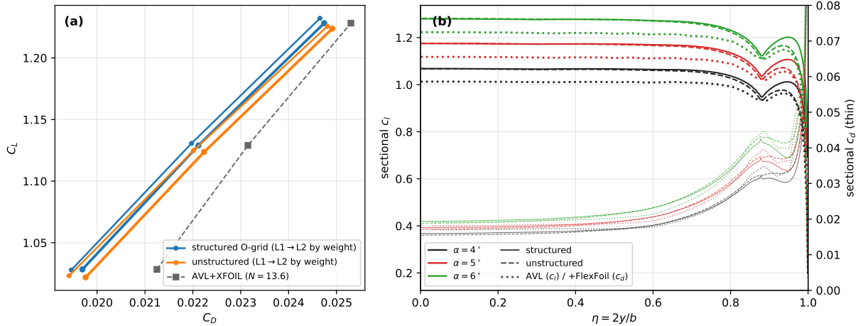
Figure 24: Daedalus polar and sections. Families agree at L1 to 0.46–0.53% in C_L and 0.4–1.6 counts in C_D , at L0 to 0.74–0.97% and 18–21 counts; taper break at \eta = 0.88 .
