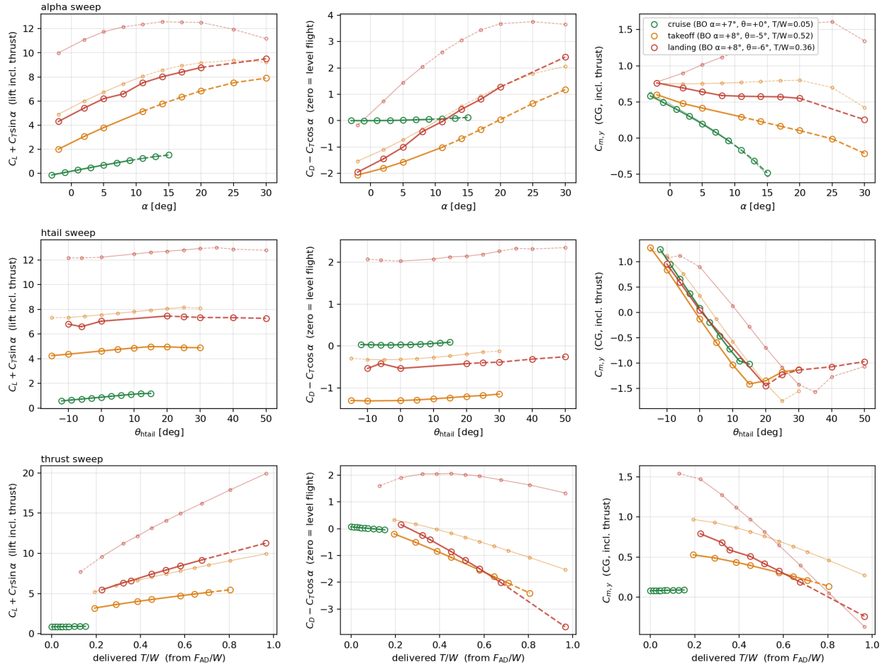
Fig. 5 Sensitivity sweeps for the gap-high configuration (Step 2; large circles, thick lines ) with the cont-high baseline of Fig. 4 overlaid ( small circles, thin lines, same colors ). Same axes, color encoding, and C_{L,total}/C_{D,total} convention as Fig. 4. The flap gap stabilises every phase relative to cont-high: cruise stays high (+51.6%), takeoff swings from neutral ( \approx 0 in cont-high) to weakly stable ( = +12.1\% ), and landing flips from strongly unstable ( = -23.8\% in cont-high) to weakly stable ( = +6.8\% ). Mechanism: streamwise vortices at the flap-segment edges roll the inboard prop wake inboard along the wing-trailing- edge gap, producing a coherent upwash column that impinges on the lower surface of the horizontal tail; local d\epsilon/d\alpha at the htail station effectively flips sign relative to the continuous-flap configuration, steepening the htail’s restoring moment.
