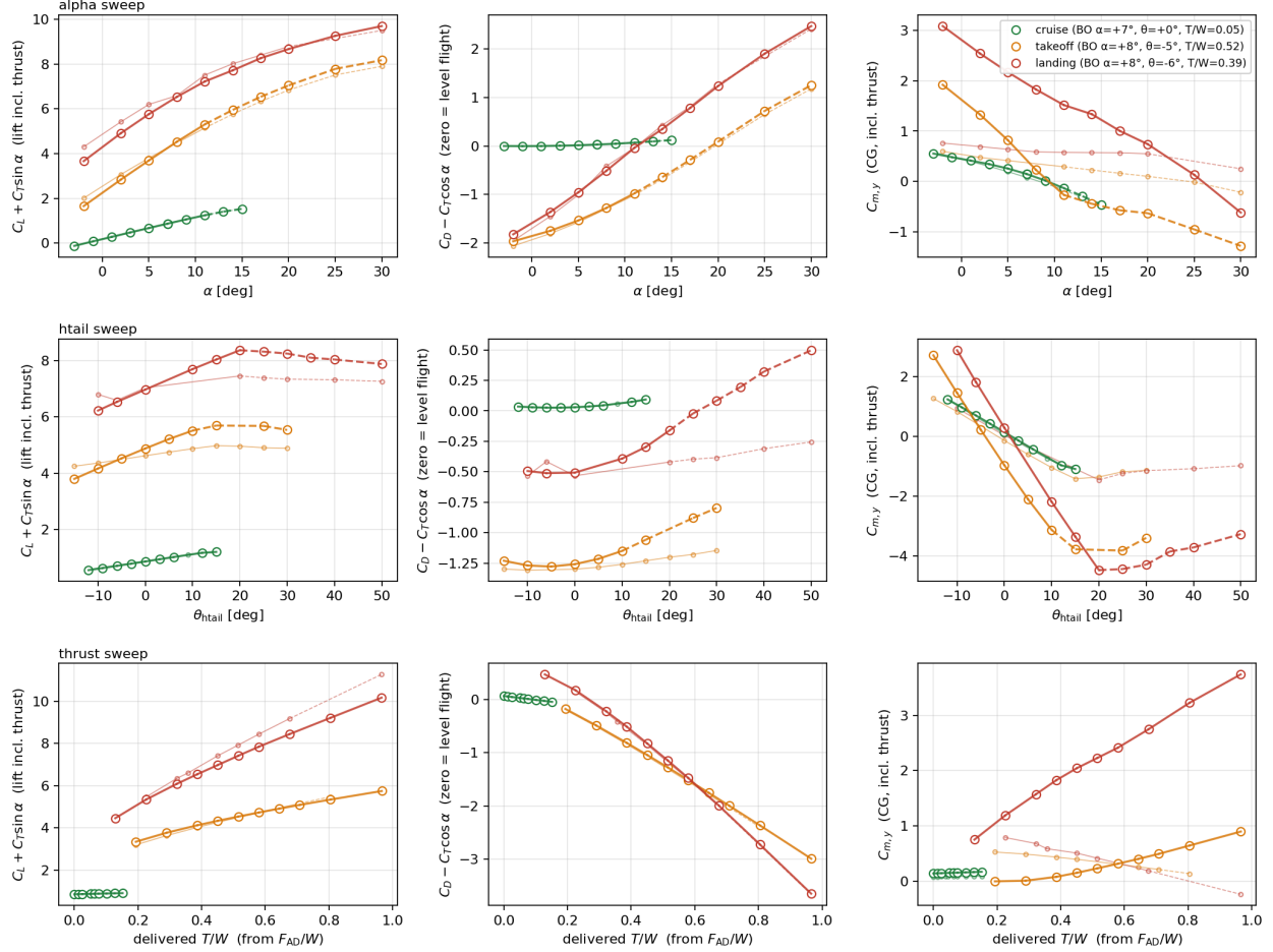
Fig. 6 Sensitivity sweeps for the gap-low configuration (Step 3; large circles, thick lines ) with the gap-high baseline of Fig. 5 overlaid ( small circles, thin lines, same colors ). Same axes, color encoding, and C_{L,total}/C_{D,total} convention as Fig. 4. All three phases of gap-low are strongly stable: the C_{mCG} -vs- \alpha slopes (third column) are sharply negative and the elevator- authority slopes ( \partial C_{mCG}/\partial \theta_{ht} , middle row, third column) are roughly doubled relative to cont-high. The htail is in the prop slipstream and benefits from a 4–9 \times dynamic-pressure boost. Reading C_{D,total} in the thrust-sweep row (bottom-middle) gives a direct visualisation of the level-flight thrust setting at each phase: the C_{D,total} = 0 crossing identifies the trimmed level-flight thrust setting at that phase’s airspeed.
