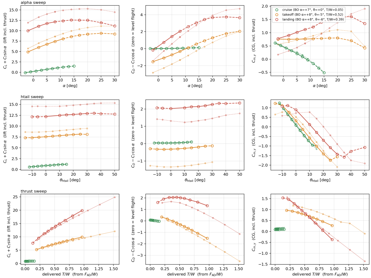
Fig. 4 Sensitivity sweeps for the cont-high T-tail baseline (Step 1; large circles, thick lines ), with the previous-step cont-low data of Fig. 3 overlaid ( small circles, thin lines, same colors ) for direct visual comparison of the design change. Three flight phases on common axes: cruise (green), takeoff (orange), landing (red). Rows are the three sensitivity sweeps ( \alpha , \theta_{ht} , T/W ); the first two columns are C_{L,\text{total}} = C_L + C_T \sin \alpha and C_{D,\text{total}} = C_D - C_T \cos \alpha , so C_{D,\text{total}} = 0 corresponds to level flight. Solid line segments lie inside the linear-fit range; dashed segments lie outside. Cruise (SM = +55%) is stable, takeoff (SM \approx 0%) is neutrally stable, and landing (SM = -24%) is strongly unstable despite the 40%-span, full-chord, high-mounted horizontal stabiliser.
