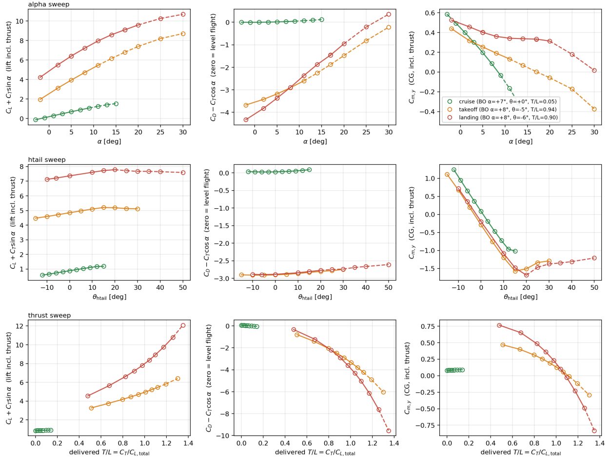
Fig. 7 Sensitivity sweeps for the gap-high configuration (Step 2). Same axes, color encoding, and C_{L,total}/C_{D,total} convention as Fig. 5. Compared with the cont-high baseline, the flap gap stabilises takeoff and landing: takeoff goes from weakly stable to moderately stable, and landing flips from mildly unstable to weakly stable – numbers in Table 1. Mechanism: streamwise vortices at the flap-segment edges roll the inboard prop wake inboard along the wing-trailing-edge gap, producing a coherent upwash column that impinges on the lower surface of the horizontal tail; local d\epsilon/d\alpha at the htail station effectively flips sign relative to the continuous-flap configuration, steepening the htail’s restoring moment.
