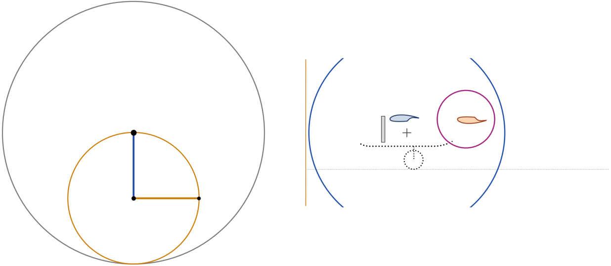
Fig. 13 Four-cylinder robot-arm topology. Left: world-frame workspace overview; freestream is along +x from the left edge. Cyl 1 (shoulder, grey) and cyl 2 (elbow, orange) form the translating 2-link arm ( L_1 = L_2 = 750 c_w ); their links are drawn as blue and orange line segments; black dots mark joints. Right: airframe-scale side view in body frame (origin at CG, +x toward tail, +z up). Solid shapes are the geometry meshed in CFD: wing at x \in [-0.5, +0.5] c_w , htail at [+1.5, +2.5] c_w , actuator disk at x = -0.7 c_w . Dotted contours (fuselage belly, landing gear, ground) are schematic context not present in the simulation. Cyl 3 (airframe-pitch, blue) is a circle of radius 2.9 c_w centred at the CG – visible as two near-vertical arcs at x \approx \pm 2.9 c_w . Cyl 4 (htail-pitch, magenta) is a circle of radius 0.85 c_w centred at the htail c/4 ( x = +1.75 c_w ), giving a 0.10 c_w design gap between htail TE and cyl 4 on the +x side. Cyl 2's outer boundary closest to the body lies on the nose side, drawn as the orange arc at x \approx -3 c_w , 0.10 c_w outside cyl 3 there. Cyl 1's nearest body-frame boundary point is \sim 313 c_w off the airframe and cannot be drawn at this scale; see the left panel.
