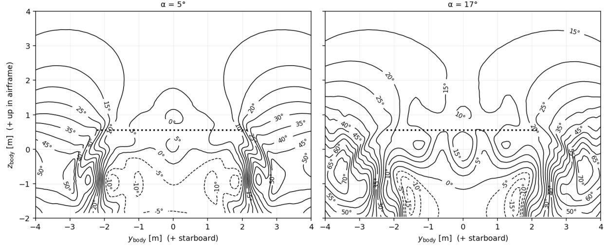
Fig. 10 Wind-frame downwash \epsilon at the gap-low htail station, \alpha = +5^\circ and +17^\circ ; same slice and conventions as Fig. 4. The low htail position is recovered ironically: the gap-upwash column reaches the htail span, and the slipstream column lifts local u_{\text{world}} to \approx 2 V_\infty . Combined, these give the large-margin landing SM and the \approx 2\times elevator-authority boost in Table 1.
