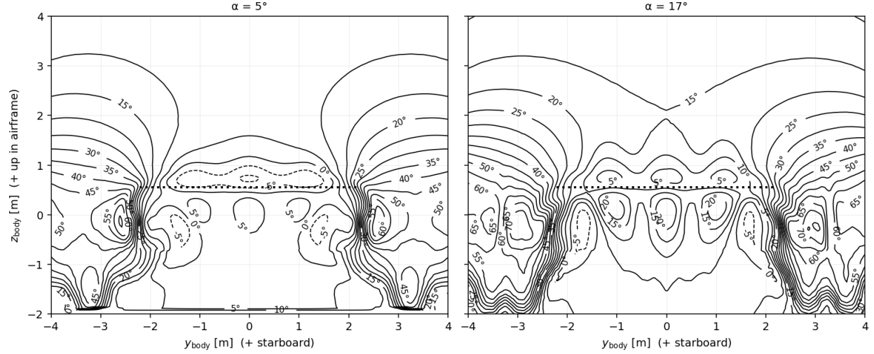
Fig. 12 Wind-frame downwash \epsilon at the v3 htail station ( x_b = \text{htail LE} - 0.23 \text{ m} , v3 BO landing trim), \alpha = +5^\circ and +17^\circ ; conventions as Fig. 4. The shortened boom retains the gap-upwash column and the slipstream acceleration at the htail station; combined with the 0.53\times moment arm this gives the v3 trim headroom of Fig. 11.
