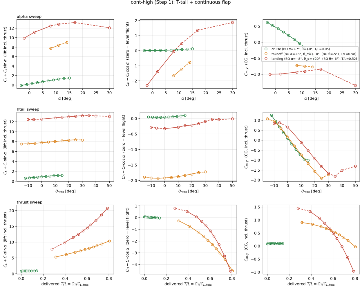
Fig. 5 Sensitivity sweeps for the cont-high T-tail baseline (Step 1), three flight phases on common axes: cruise (green), takeoff (orange), landing (red). Rows are the three sensitivity sweeps ( \alpha , \theta_{ht} , T/L ); the first two columns are C_{L,total} = C_L + C_T \sin \alpha and C_{D,total} = C_D - C_T \cos \alpha , so C_{D,total} = 0 corresponds to level flight. Solid line segments lie inside the linear-fit range; dashed segments lie outside. See Table 1 for the static-margin entries.
