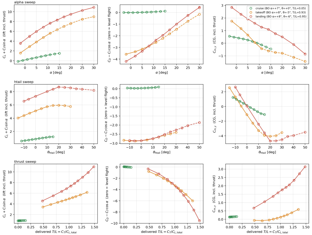
Fig. 9 Sensitivity sweeps for the gap-low configuration (Step 3). Same axes, color encoding, and C_{L,total}/C_{D,total} convention as Fig. 5. All three phases of gap-low are strongly stable: the C_{mCG} -vs- \alpha slopes (third column) are sharply negative and the elevator- authority slopes ( \partial C_{mCG}/\partial \theta_{ht} , middle row, third column) are roughly doubled relative to cont-high. The htail is in the prop slipstream and benefits from a 4–9 \times dynamic-pressure boost. Reading C_{D,total} in the thrust-sweep row (bottom-middle) gives a direct visualisation of the level-flight thrust setting at each phase: the C_{D,total} = 0 crossing identifies the trimmed level-flight thrust setting at that phase’s airspeed.
