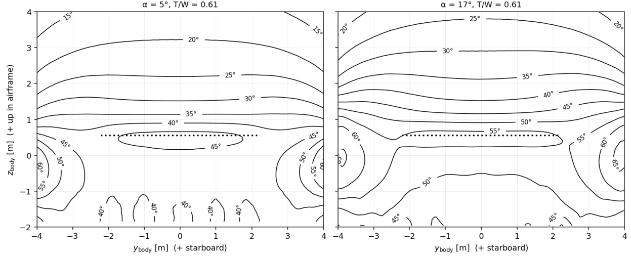
Fig. 4 Wind-frame downwash \epsilon at the cont-low htail station ( x_b = \text{htail LE} - 0.45 \text{ m} , landing trim, T/L \approx 0.60 ), at \alpha = +5^\circ (left) and \alpha = +17^\circ (right). Labeled contour lines are degrees of \epsilon ; the dotted black line marks the htail span at its body- z station. The htail sits inside a deep downwash column ( \epsilon \gtrsim +20^\circ ) – the geometric mechanism behind the cont-low landing instability.
