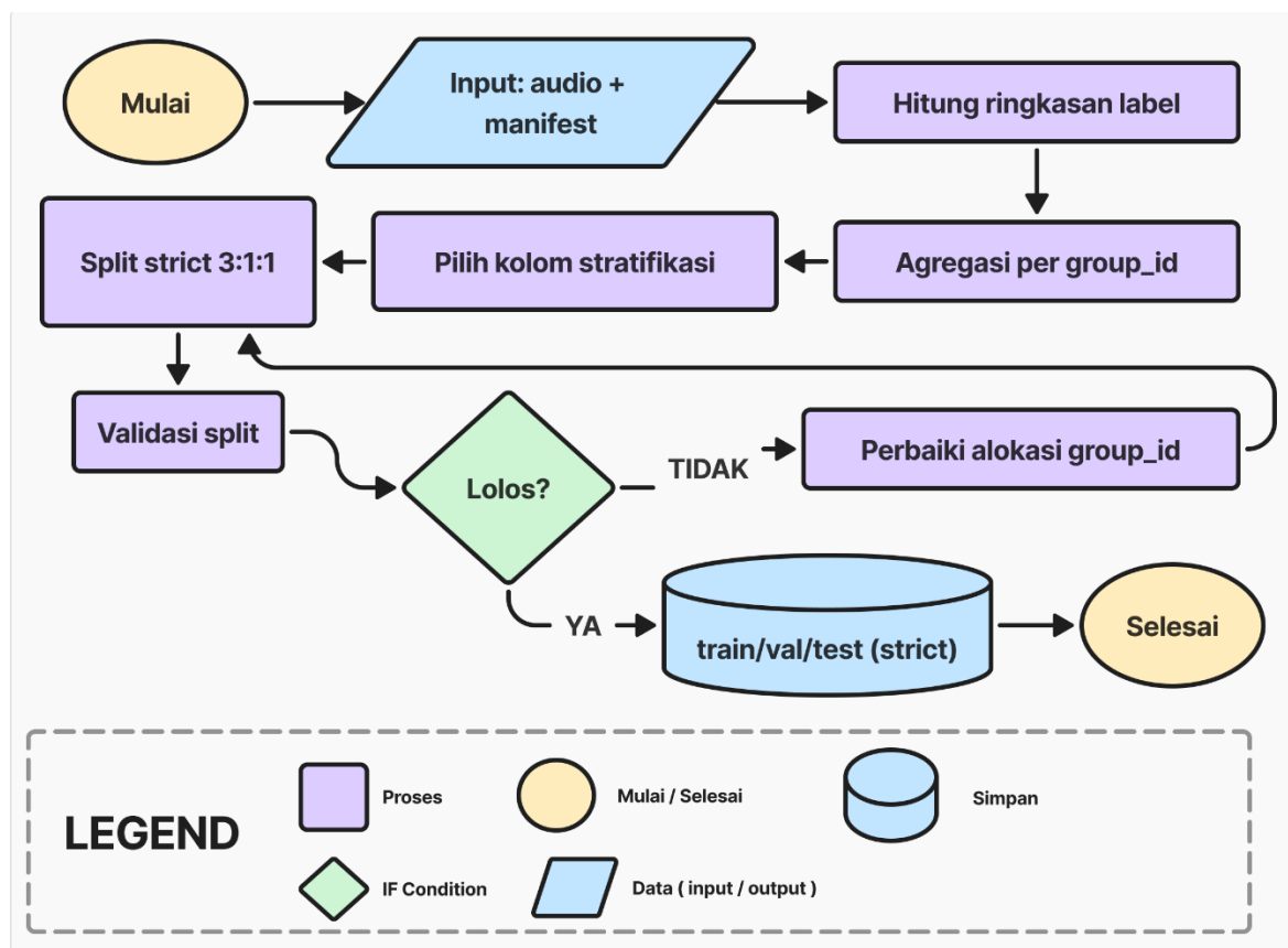
Gambar 3.3 Alur Split Strict
