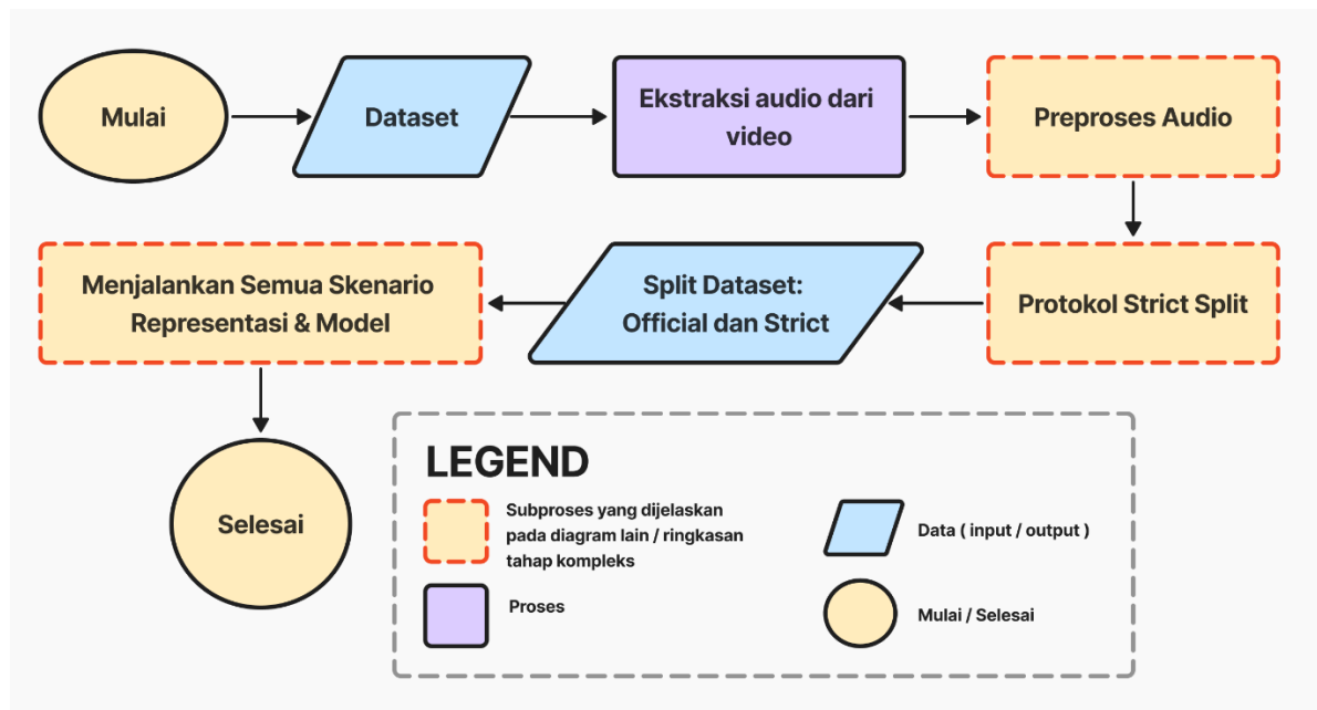
Gambar 3.1 Diagram Alir Umum Penelitian Audio-only Personality Estimation
