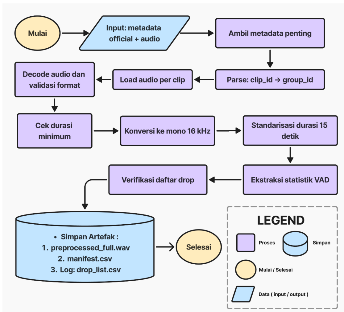
Gambar 3.2 Alur Praproses Dataset
