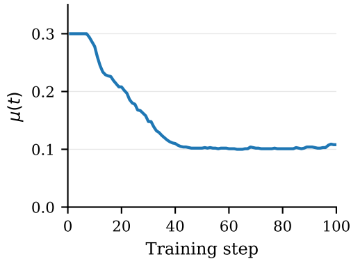
(B) Adaptive BC weight \mu(t)
