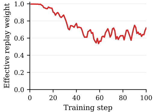
(A) Effective teacher replay weight \hat{w}_\tau
