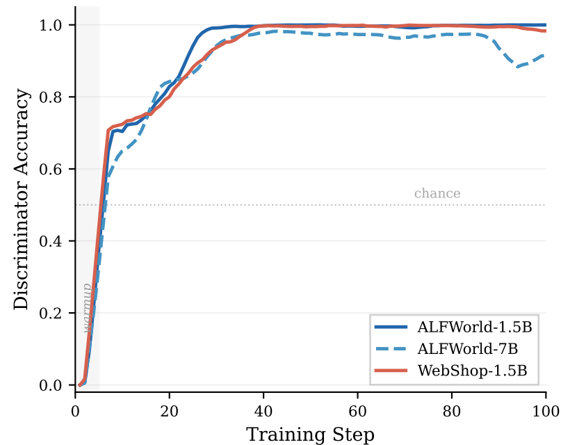
(a) DR3 Discriminator Accuracy
