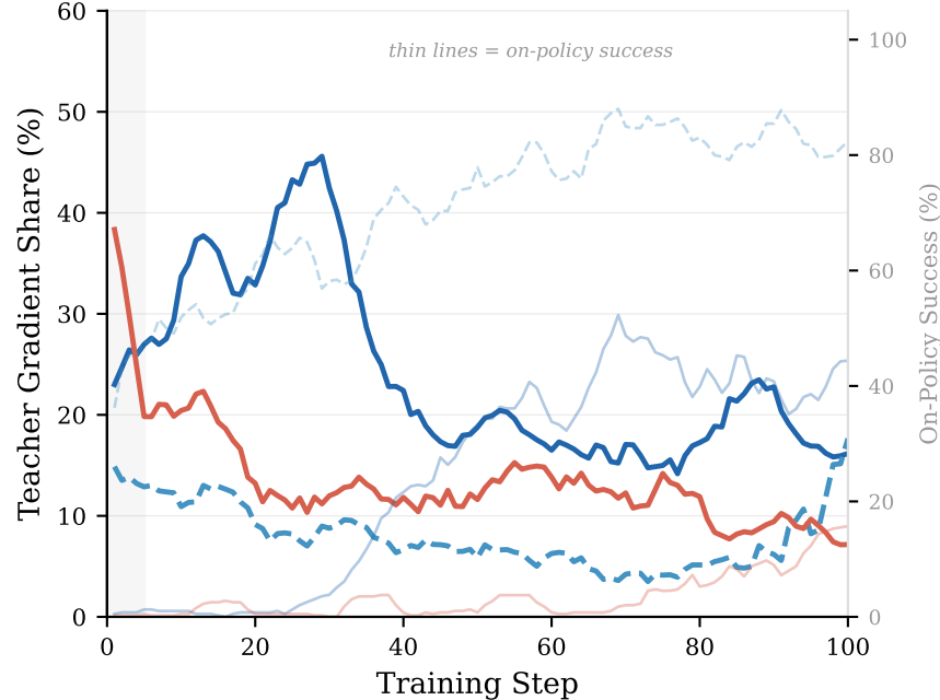
(b) Teacher Gradient Share
