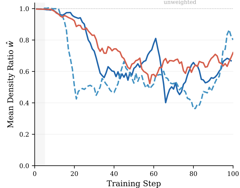
(c) Teacher Weight \hat{w}_{\text{off}}
