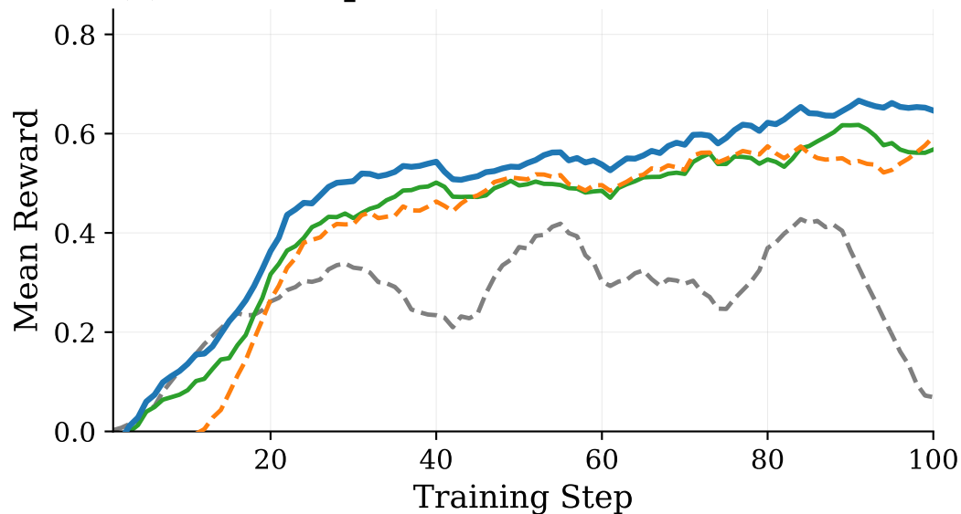
(c) WebShop 1.5B
