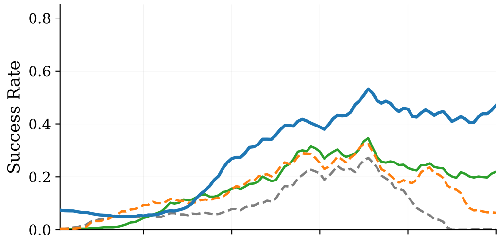
(c) WebShop 1.5B
