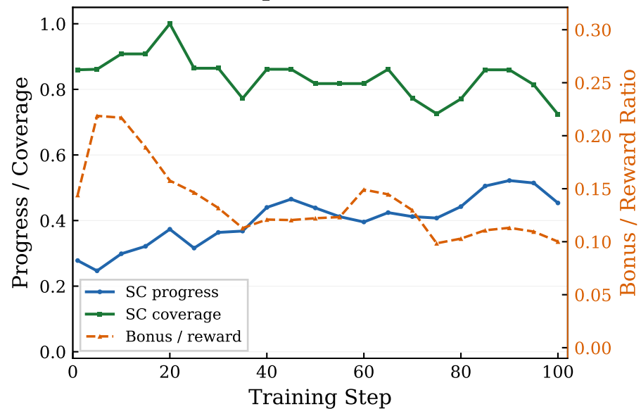
WebShop — Qwen2.5-3B
