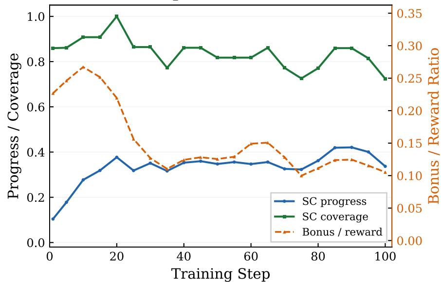
WebShop — Qwen2.5-1.5B
