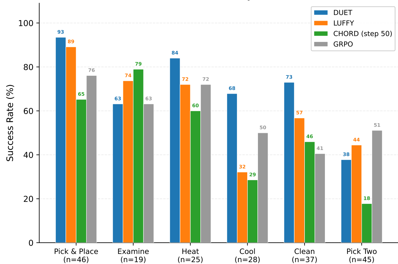
Qwen2.5-3B (step 100)
