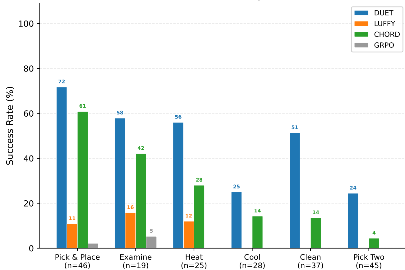
Qwen2.5-1.5B (step 100)
