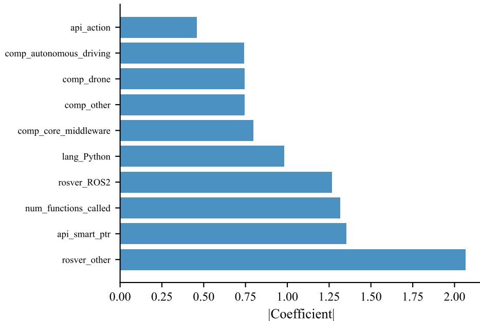
Logistic Regression
