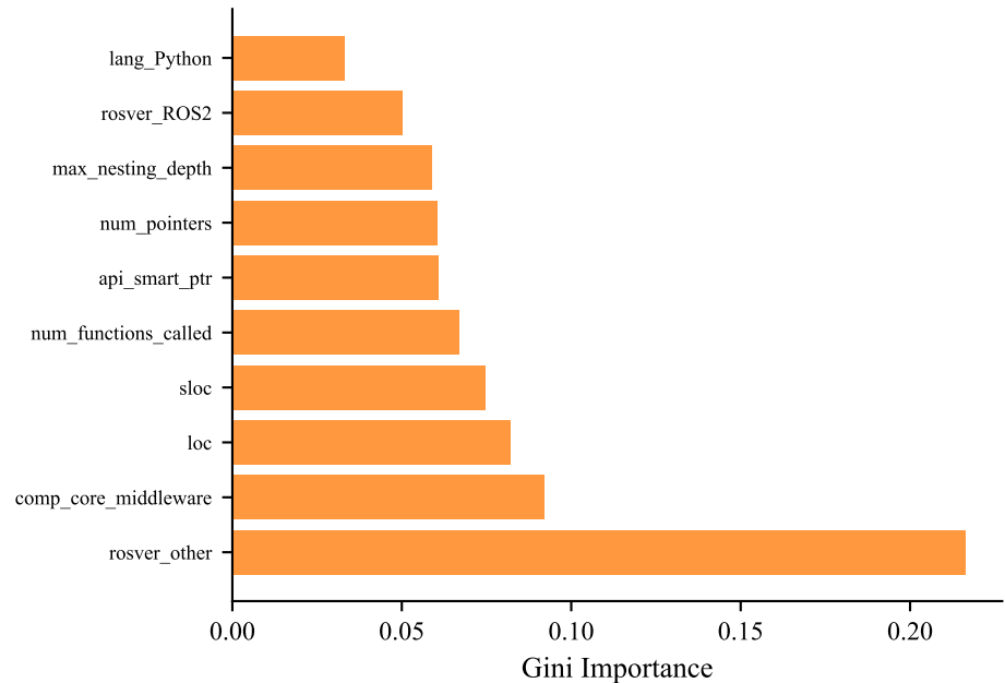
Random Forest
