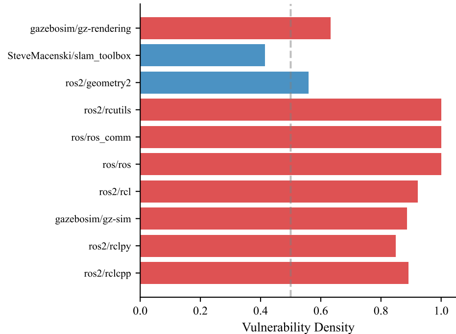
Top 10 Repos by Density
