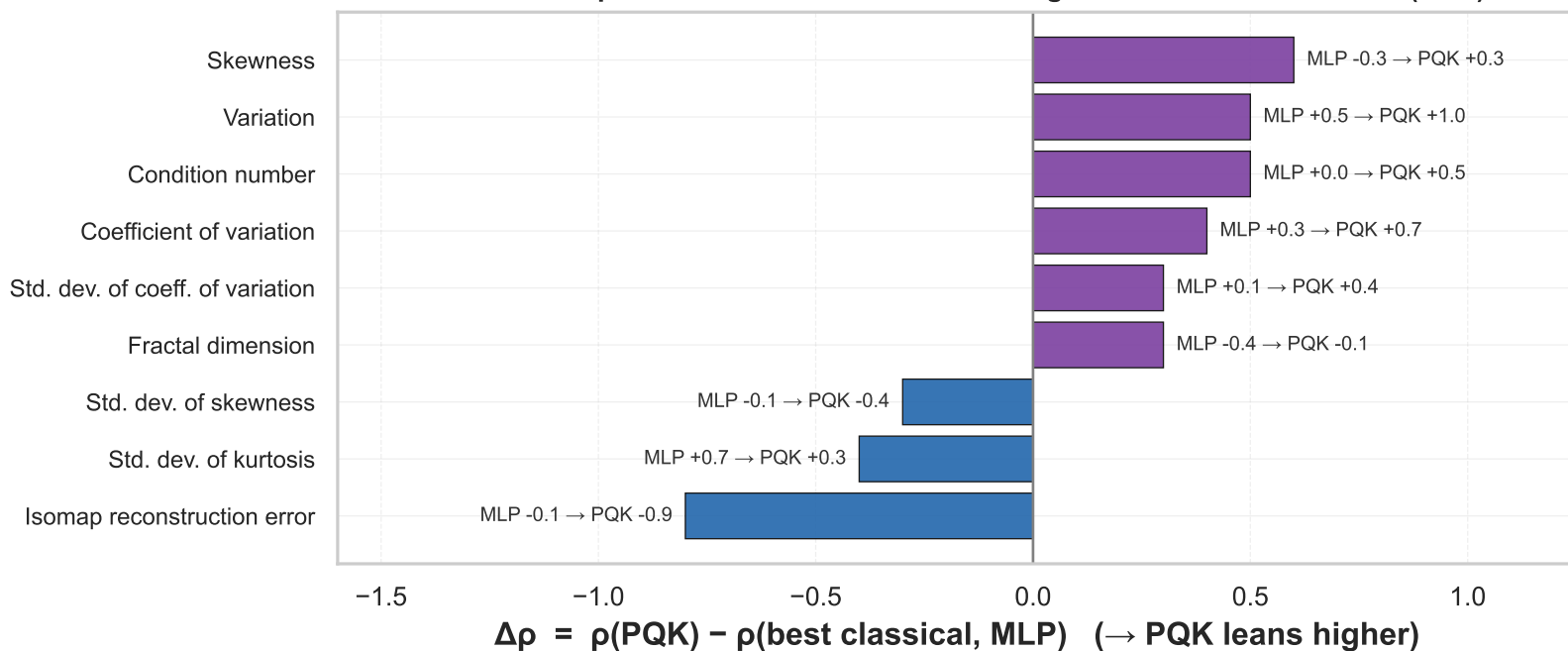
B. Where PQK's response to each characteristic diverges from the best classical (MLP)
