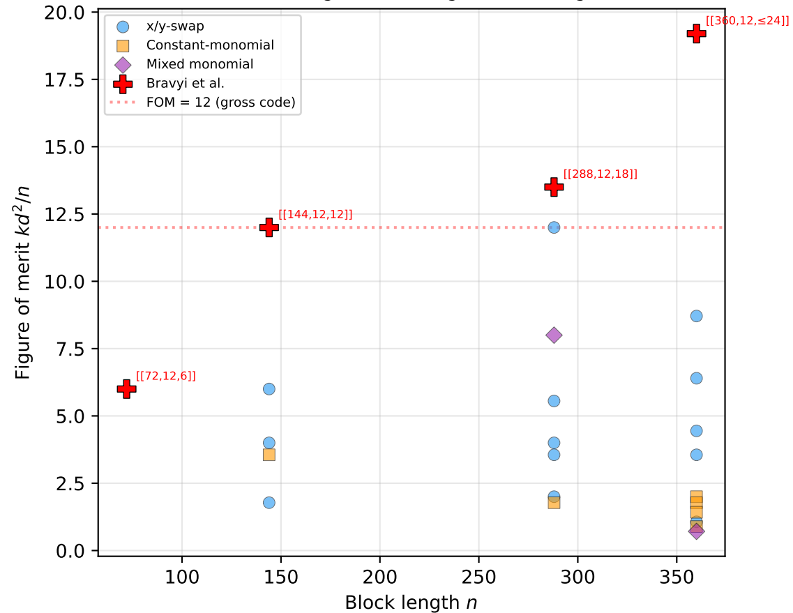
(b) FOM vs block length (CSS, weight-6 and weight-8, d \geq 4 )
