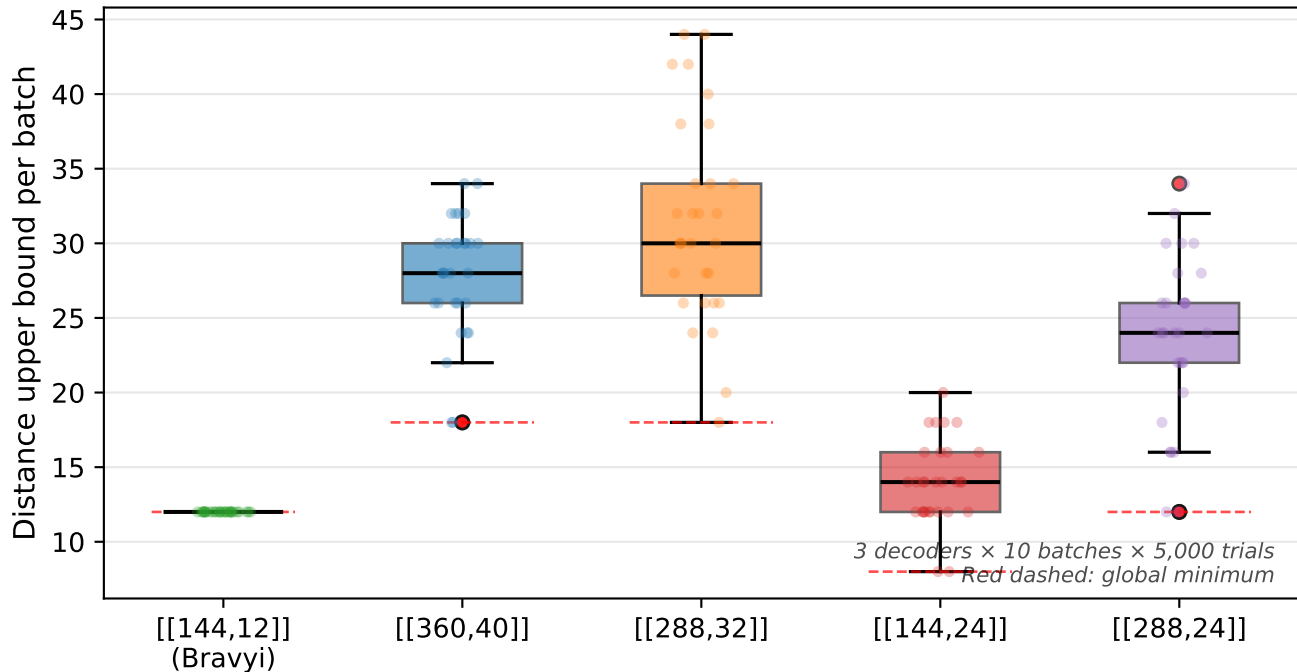
Per-batch distance distributions (150k-trial protocol)
