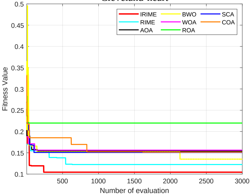
Cleveland-heart
