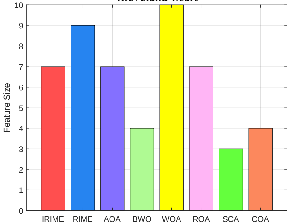
Cleveland-heart
