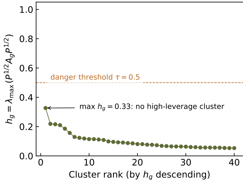
(a) leverage profile
