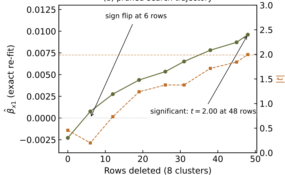
(b) pruned-search trajectory
