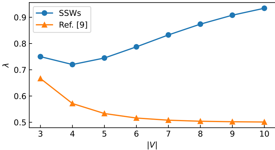
Dephasing noise
