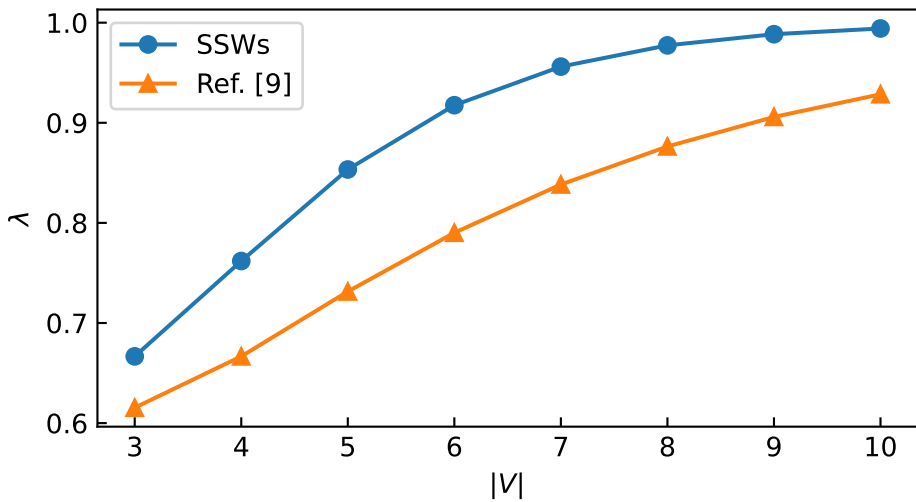
White noise
