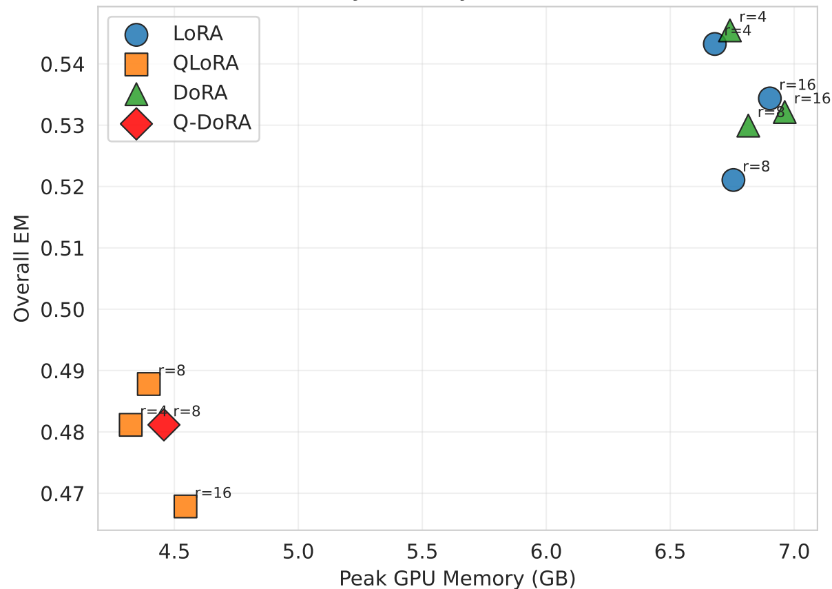
Accuracy-Memory Pareto Frontier
