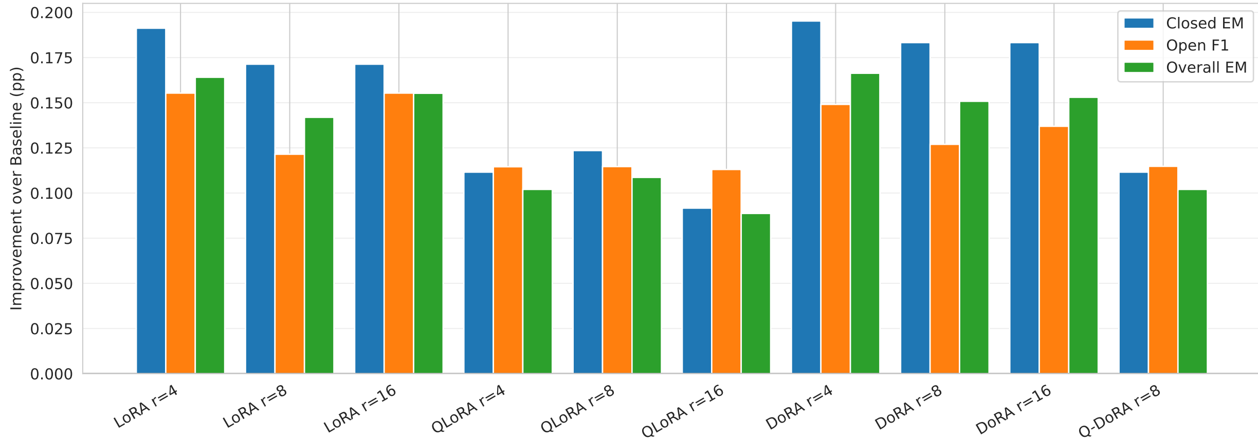
PEFT Improvement over Zero-Shot Baseline
