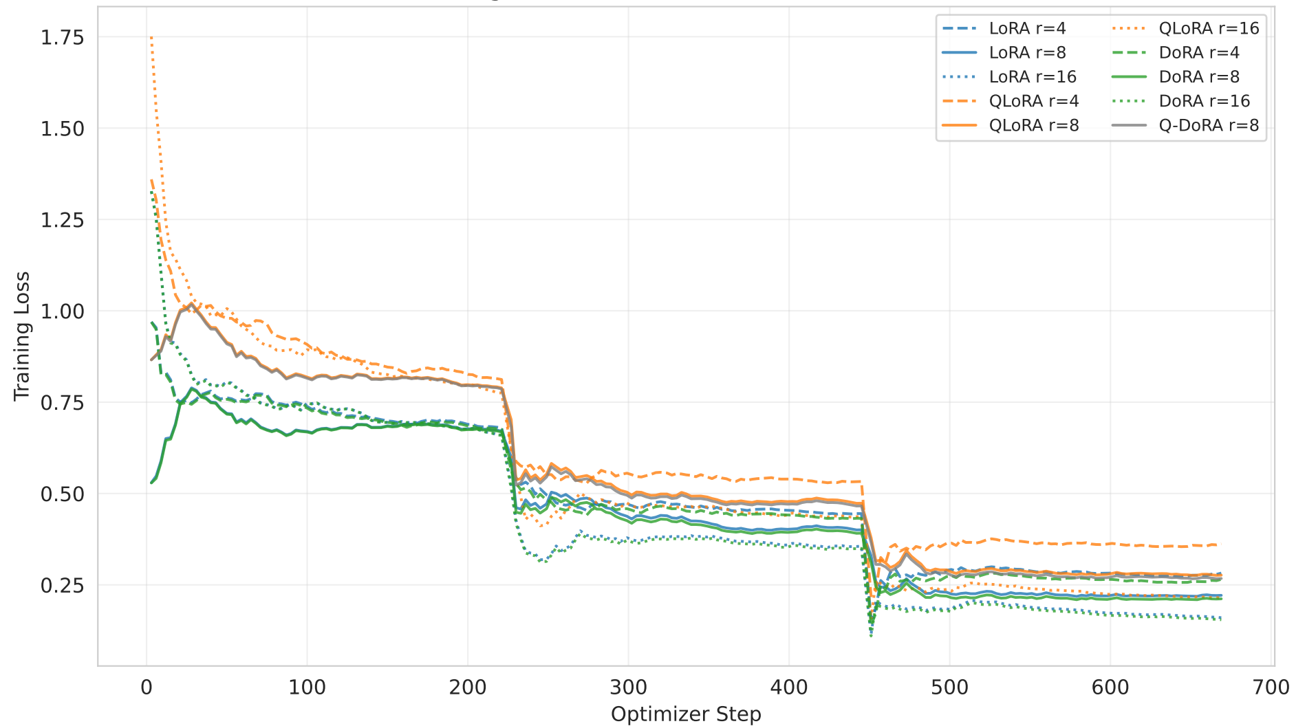
Training Loss Curves: LoRA vs QLoRA vs DoRA
