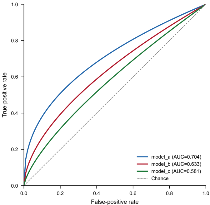
Check-in Prediction ROC
