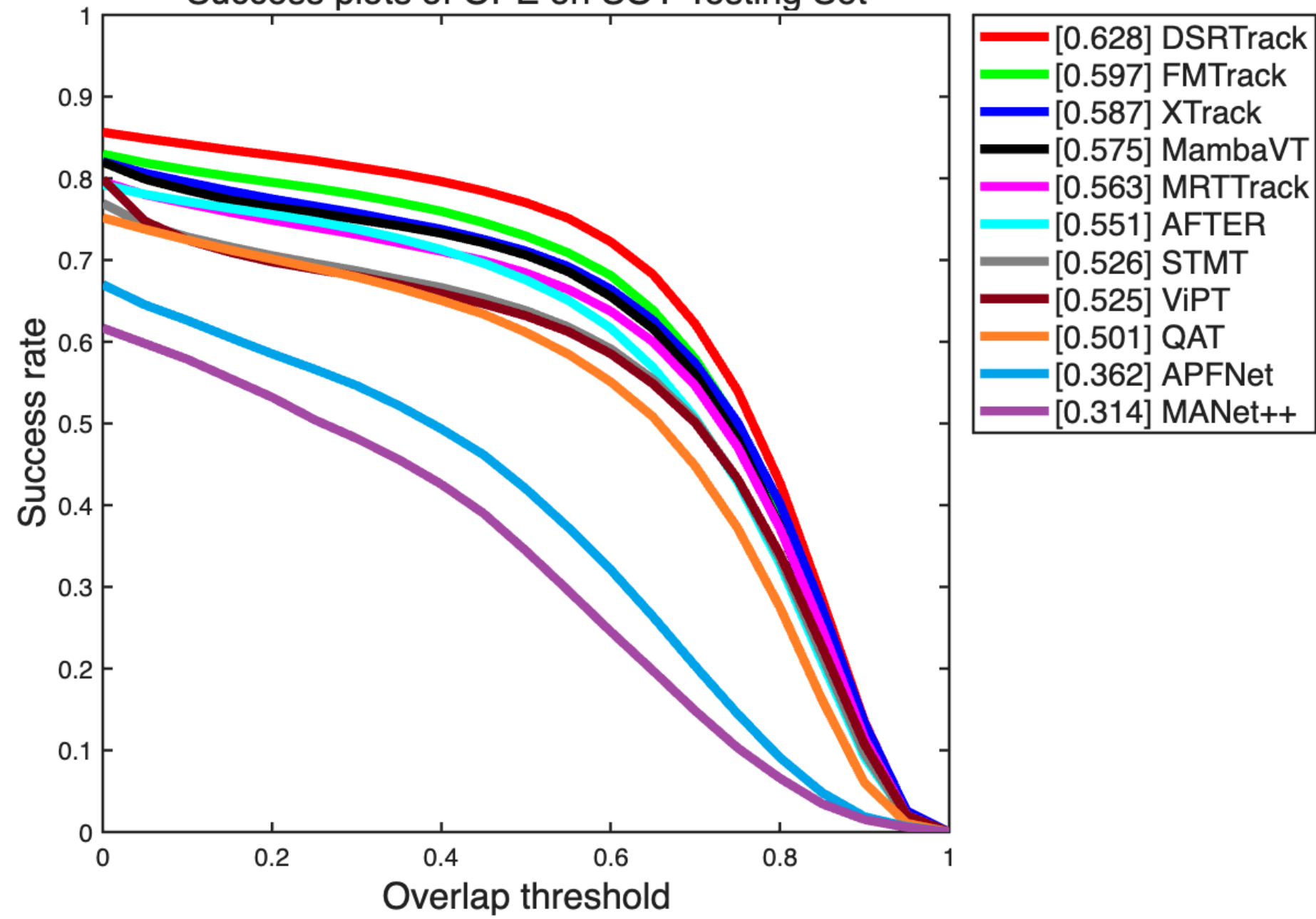
Success plots of OPE on SOT Testing Set
