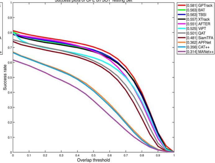
Success plots of OPE on SOT Testing Set
