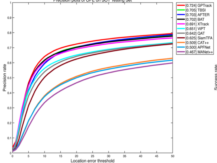
Precision plots of OPE on SOT Testing Set
