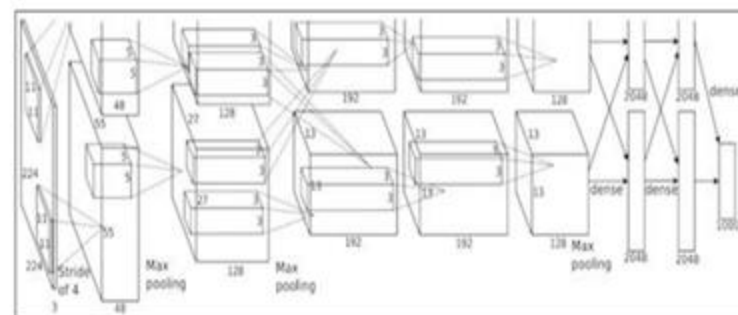
“AlexNet”
