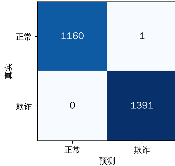
TF-IDF+LR
