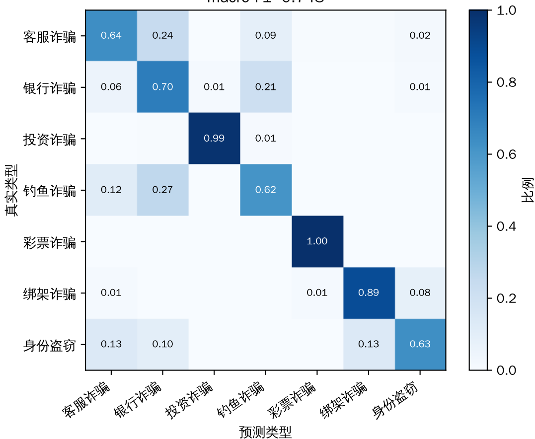
RoBERTa 欺诈类型混淆矩阵(行归一化) macro-F1=0.748
