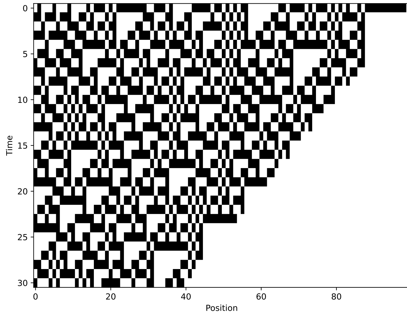
Boundary Field ( b = s \oplus \text{shift}(s) ) "Walls" (invariant under complement!)
