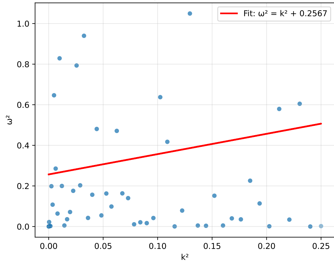
Dispersion Relation
